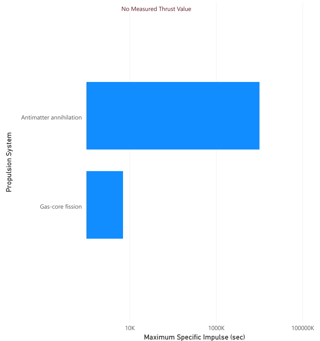
Maximum Specific Impulse per Theoretical Nuclear System
