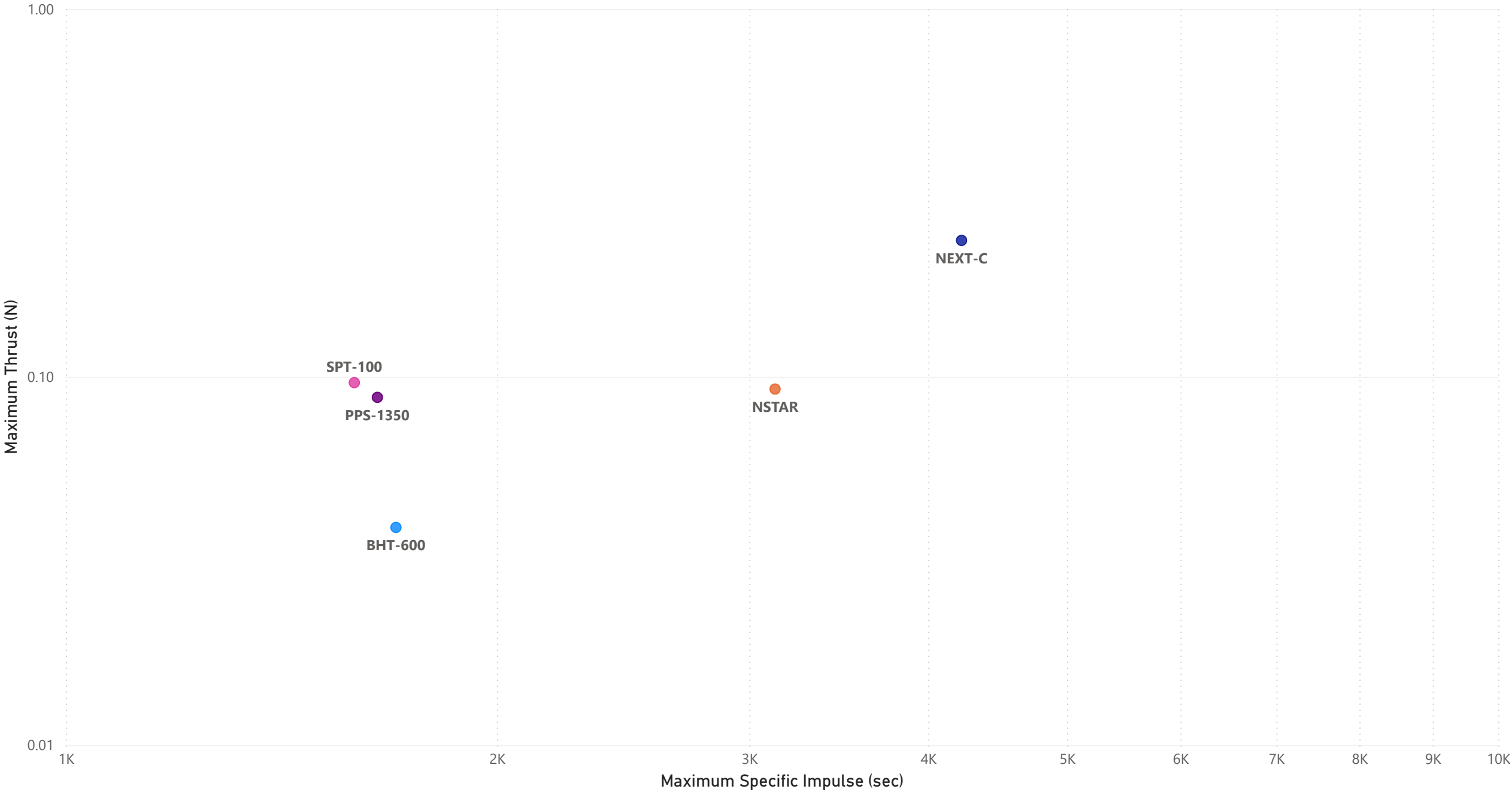
Maximum Thrust to Maximum Specific Impulse per Electric System
