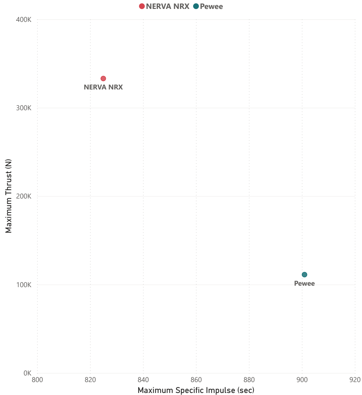
Maximum Thrust to Maximum Specific Impulse per Built Nuclear System
