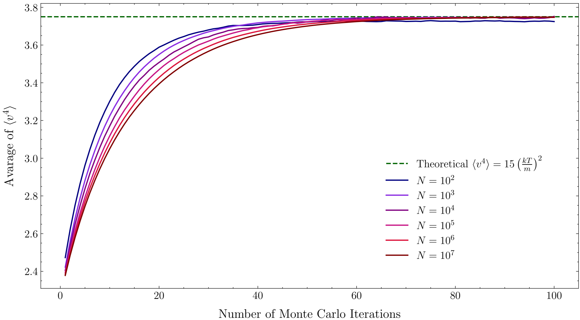
Average of \langle v^4 \rangle for different N
