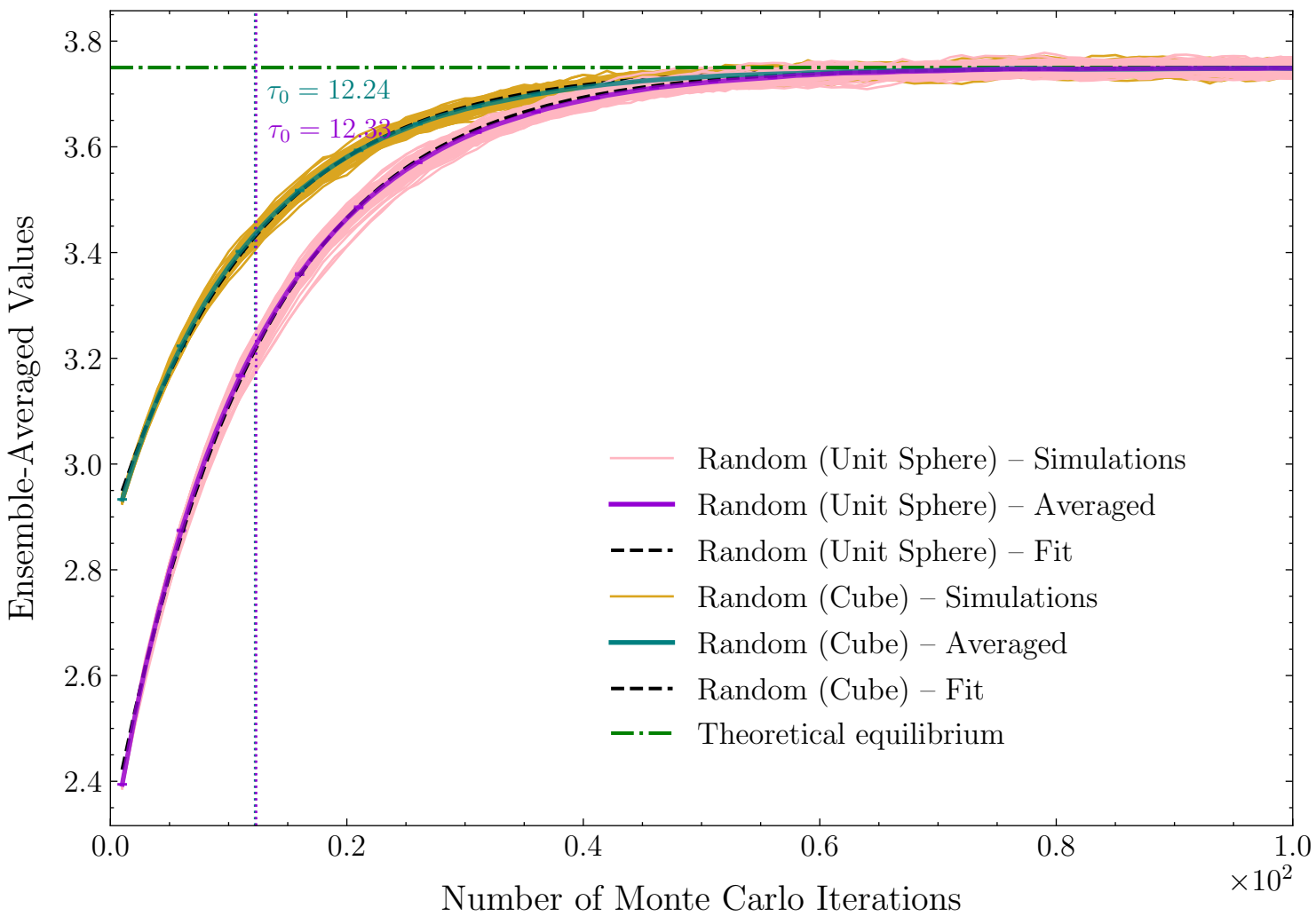
Evolution of \langle v^4 \rangle : Random Distributions in Cube vs Unit Sphere
