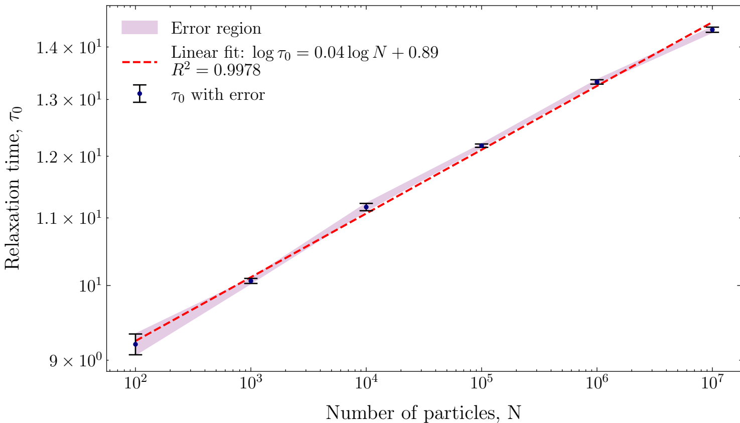
Relaxation Time \tau_0 vs Number of Particles N (Log-Log Scale)
