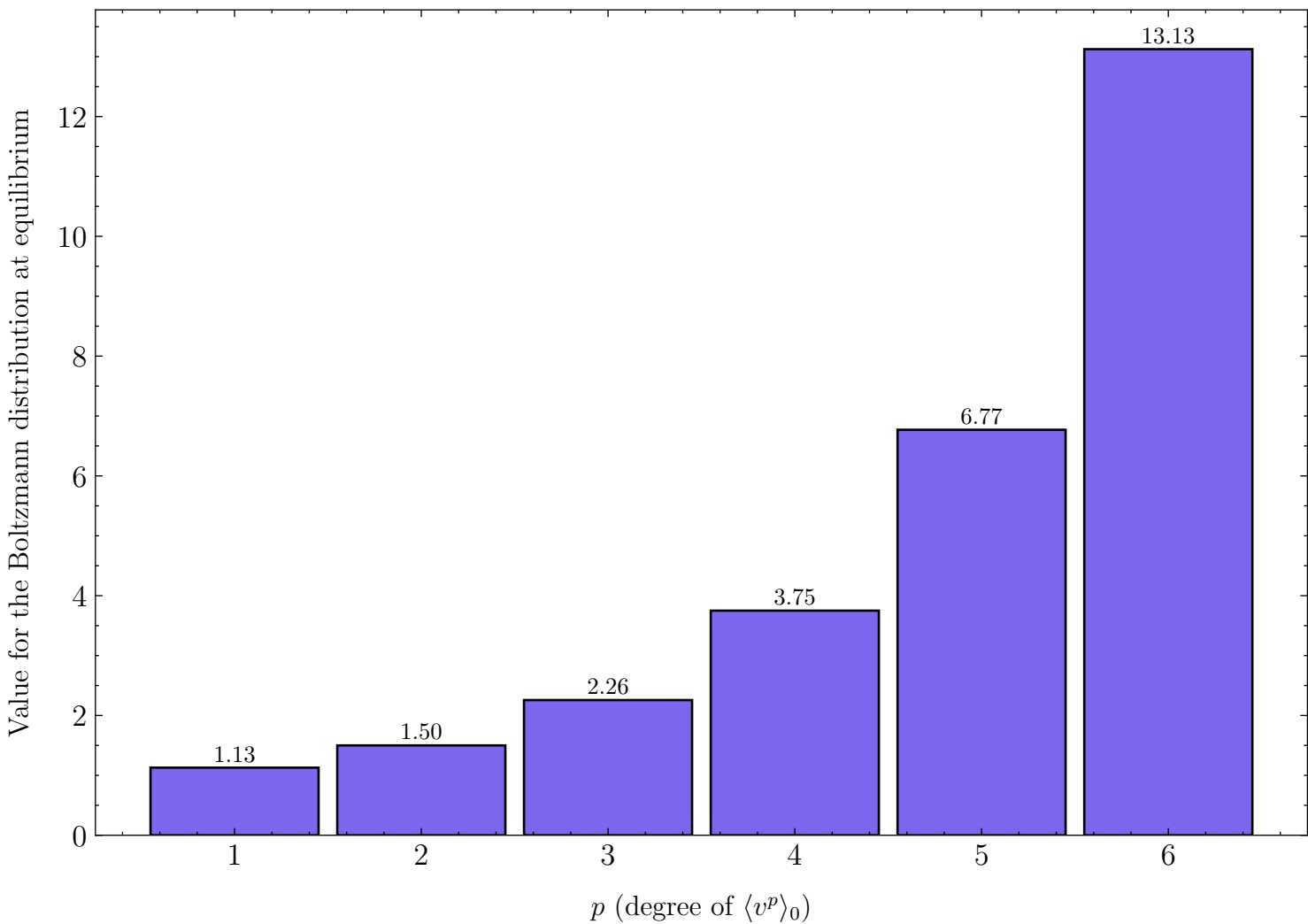
Expectation values of velocity moments for the Boltzmann distribution
