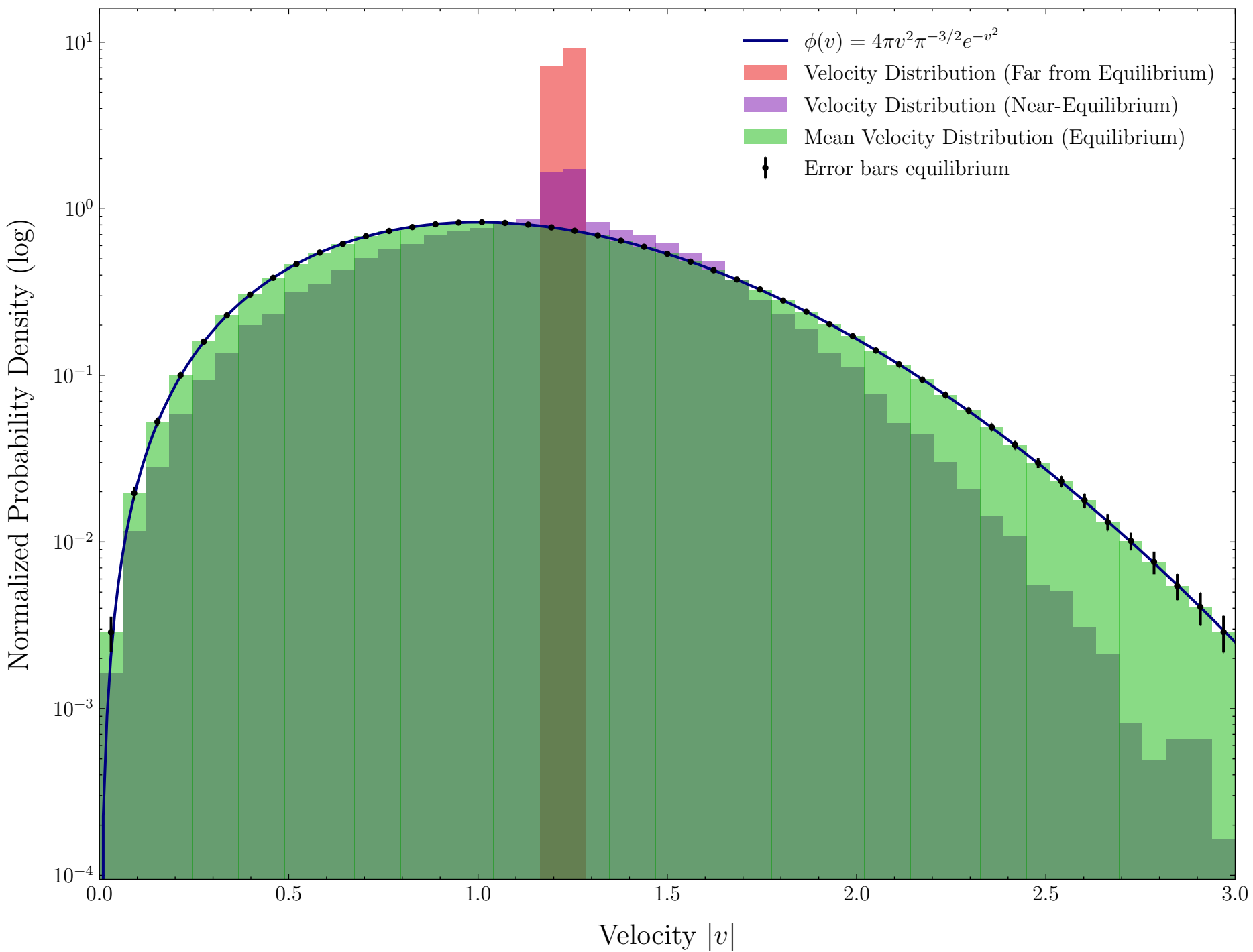
Velocity Distributions in Monte Carlo Simulation (log scale)
