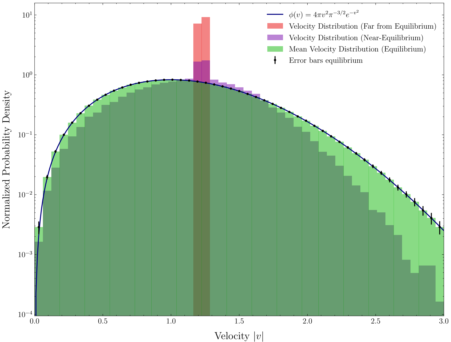
Velocity Distributions in Monte Carlo Simulation
