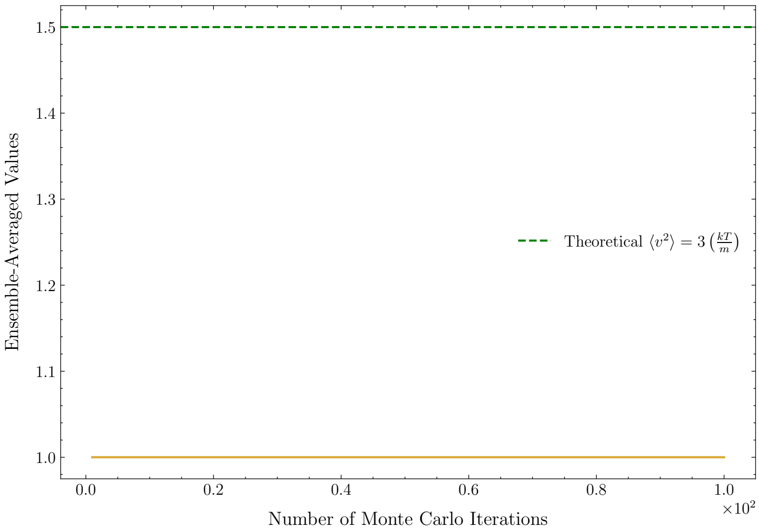
Evolution of \langle v^2 \rangle Across 100 Monte Carlo Simulations
