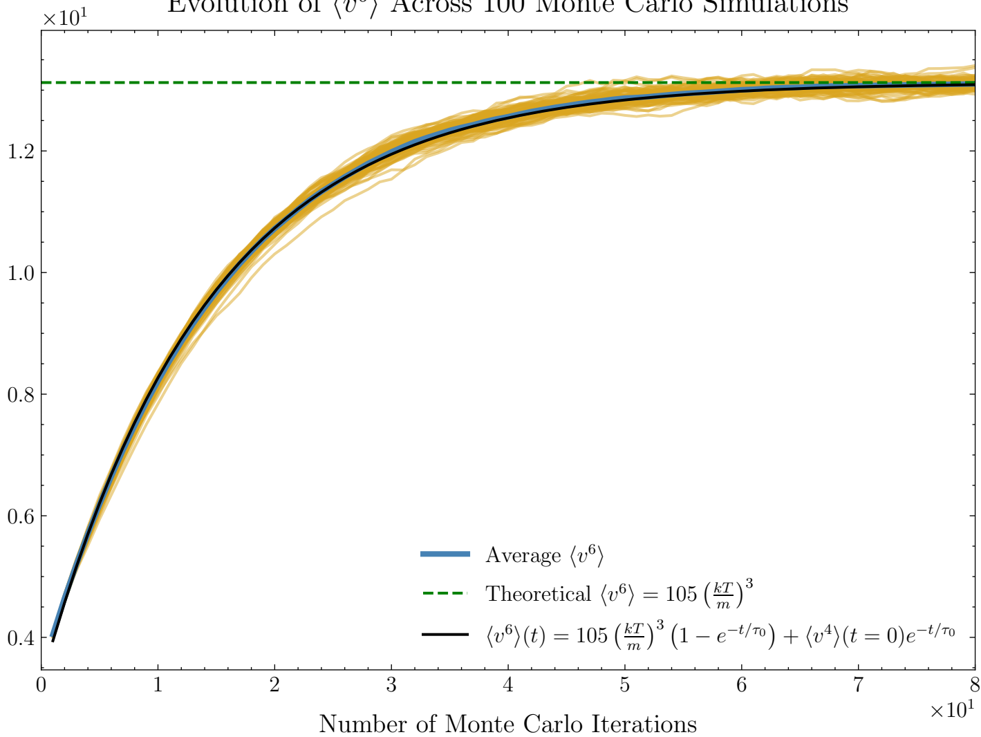
Evolution of \langle v^6 \rangle Across 100 Monte Carlo Simulations
