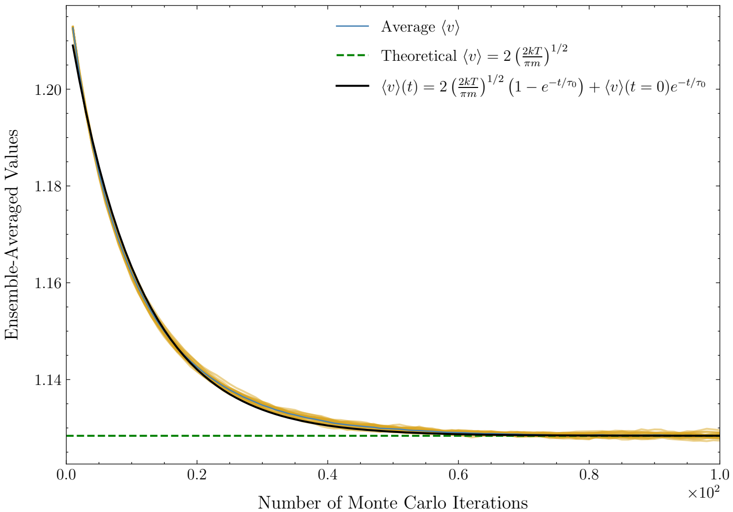
Evolution of \langle v \rangle Across 100 Monte Carlo Simulations
