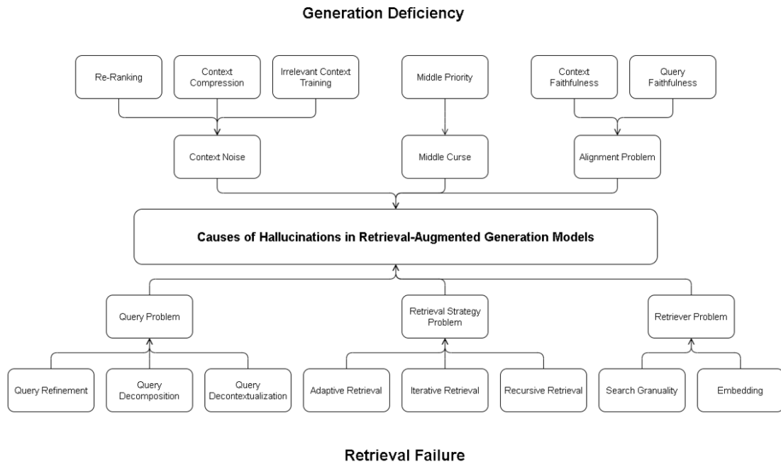
Figure 3. Causes of Hallucinations in RAG Models
