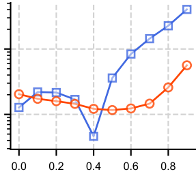
Exponent of singularity: \alpha ( G(t) \sim t^{-\alpha} )
