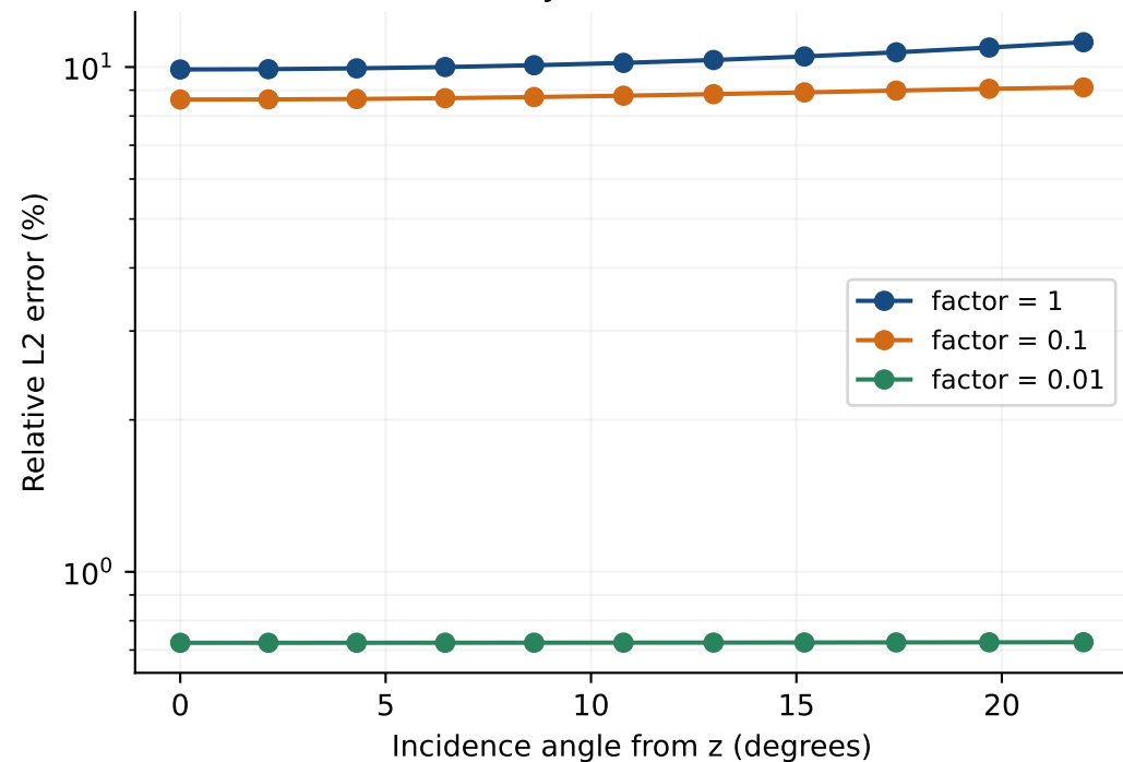
Vector Born / Maxwell full field
