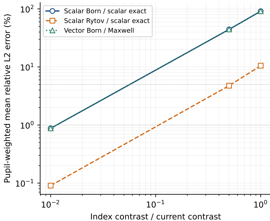
Approximation error
