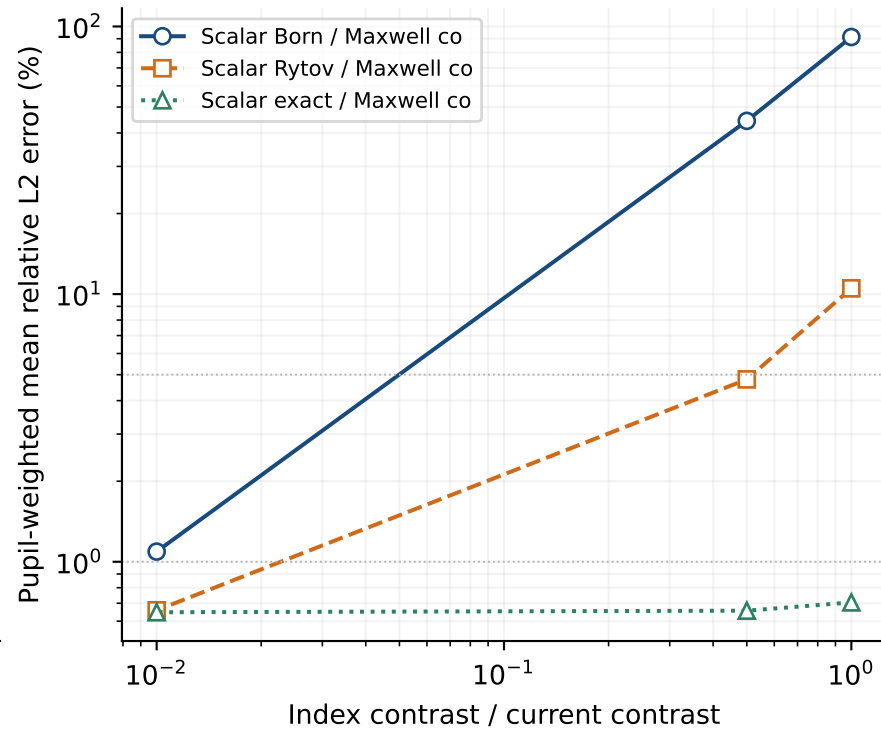
Oblate index-contrast sweep Error against Maxwell co-polarization
