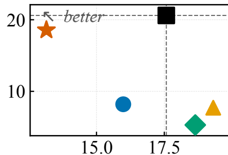
Peak request tokens (k) (c) Qwen2.5-14B — C = 8k
