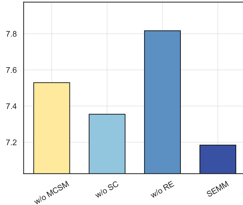
RMSE
