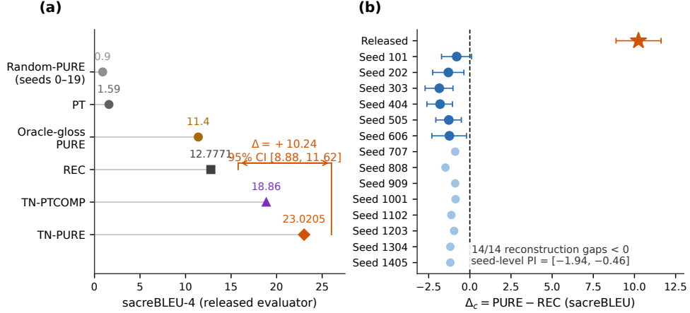
Fig. 1: Adversarial unit-test response under the released evaluator and its absence across the canonical (clip=1.0) panel. (a) System scores (sacreBLEU-4, 641-query protocol): TN-PURE 23.02 vs. REC 12.78 ( \Delta = +10.24 , post-selected), with TN-PTCOMP 18.86, PT 1.59, oracle-gloss 11.4, random-donor 0.90 ( \pm 1 SD over 20 seeds). (b) Per-checkpoint gaps: released (+10.24) vs. fourteen legacy reconstructions, all negative (donor-cluster bootstrap CIs; dispersion [-1.85, -0.80] ). The remaining families (union [-2.80, -0.36] ; full panel [-2.80, -0.21] ) are in Fig. 2; none is positive, including runs matching the released test-split competence—an absence §4.3 traces to the shared clip threshold (unclipped: +11.19).
