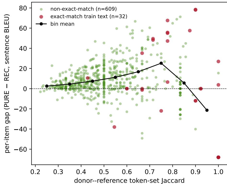
(b) Gap vs lexical donor-reference overlap
