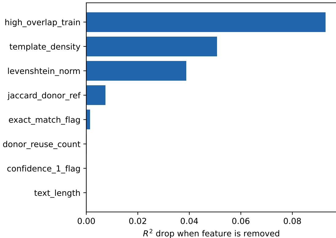
(a) Per-feature explanatory power (full R^2=0.33 )
