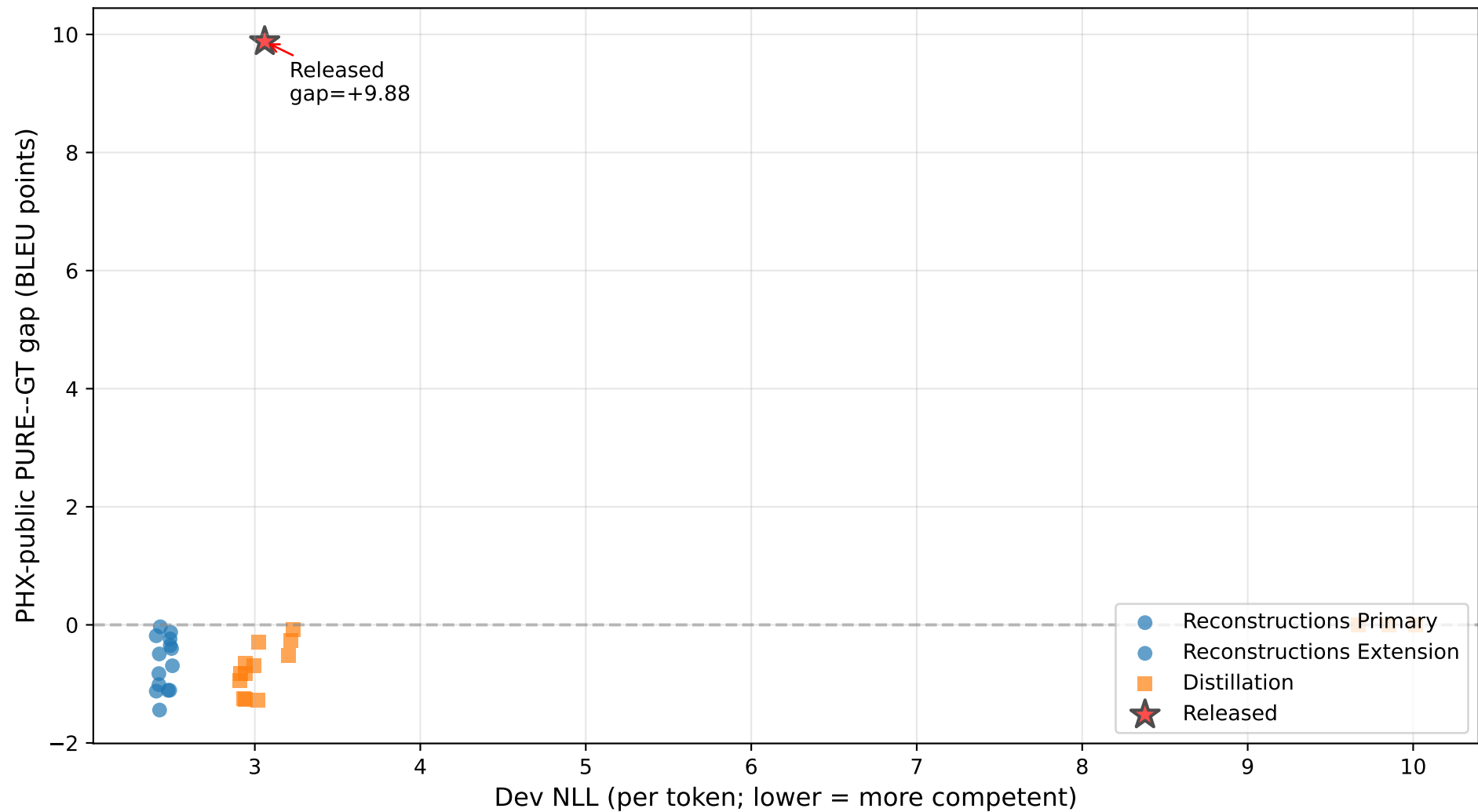
Dose-response: BT-evaluator competence vs retrieval stress-test gap (Real data; 14 reconstructions + 15 distillation students + released)
