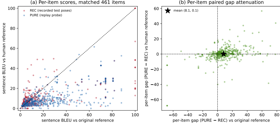
Fig. 3: Per-item reference-frame sensitivity on the matched 461-item confidence=1 subset (released evaluator, canonical hypotheses). Sentence-level sacreBLEU (0–100, same tokenizer/smoothing as corpus BLEU). (a) Per-item scores under original vs human references for REC (recorded test poses) and PURE (replay probe); the diagonal marks equal scores. PURE points sit high under the original reference and collapse toward the diagonal/low under the human reference, whereas REC points move less. (b) Per-item paired gap (PURE–REC) under original (x) vs human (y) references; the star marks the mean (sentence-level mean gap 8.11 \rightarrow 0.09, consistent in direction with the corpus-level attenuation 10.03 \rightarrow 0.95). Sentence-level means need not equal the corpus BLEU; the figure is descriptive and does not separate reference-text defects from lexical-coupling disruption or evaluator alignment.
