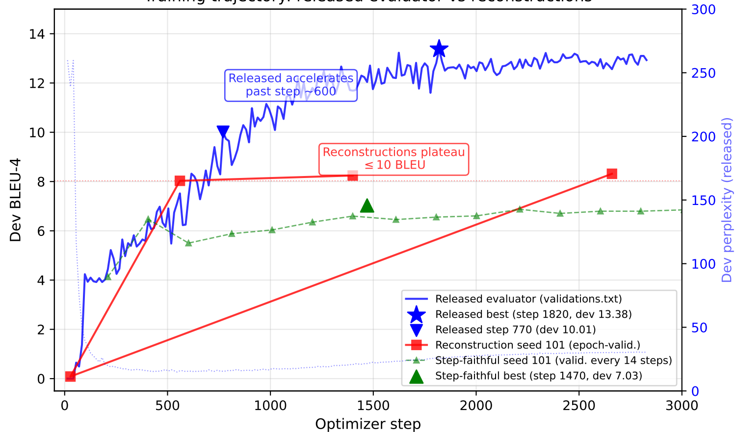
Training trajectory: released evaluator vs reconstructions
