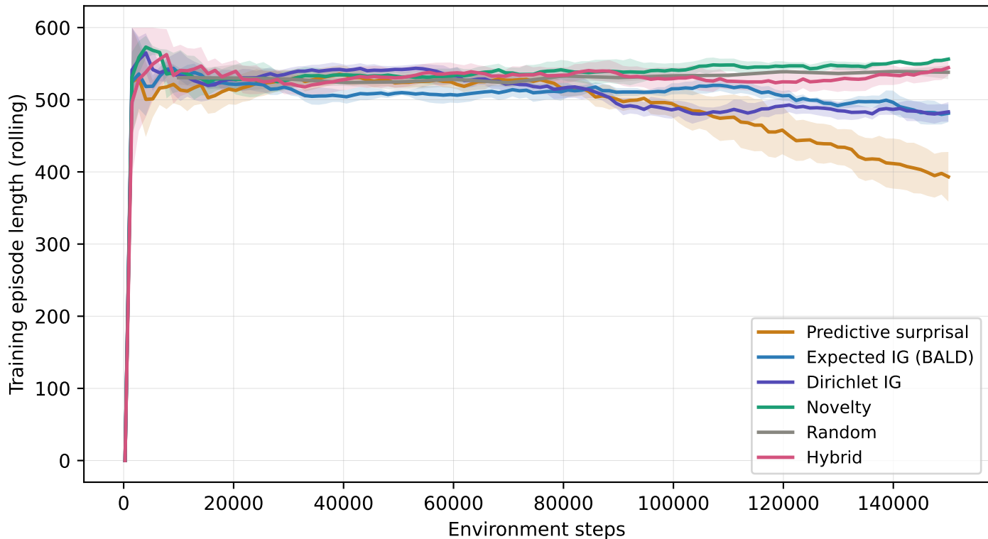
Training episode length over time (600-step budget) "rule learned → faster solving"
