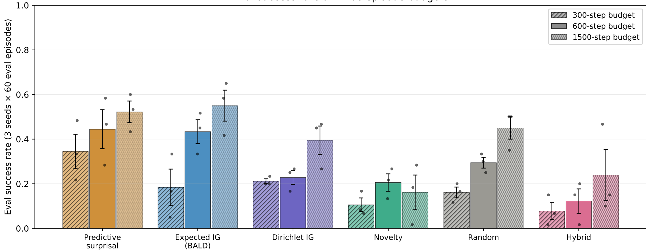
Eval success rate at three episode budgets
