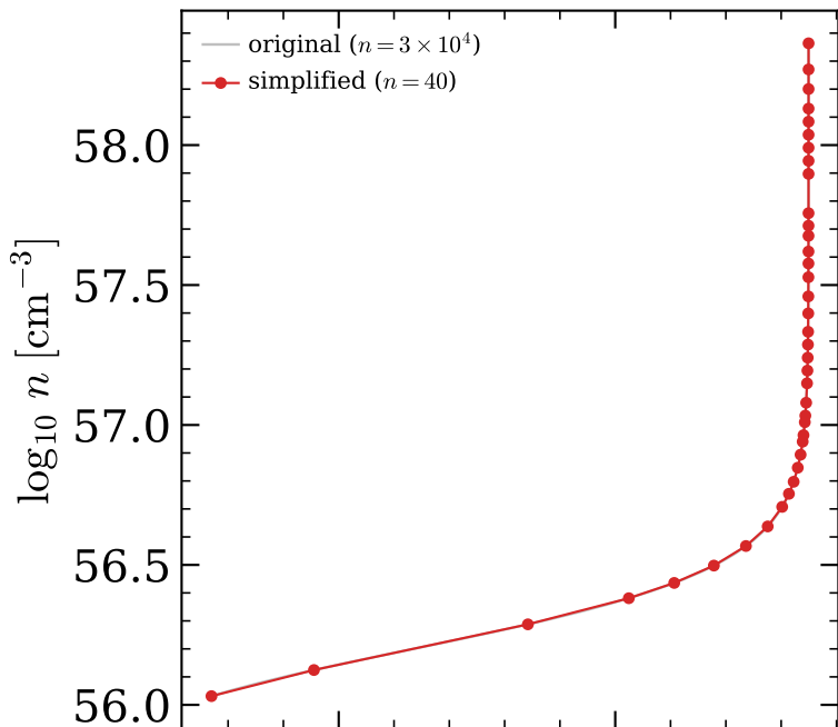
Density profile ( R^2 = 0.99999 )
