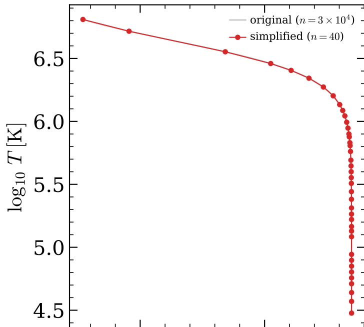
Temperature profile ( R^2 = 0.99999 )
