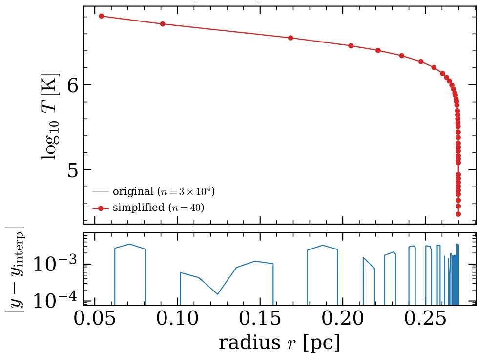
Temperature profile ( R^2 = 0.99999 )
