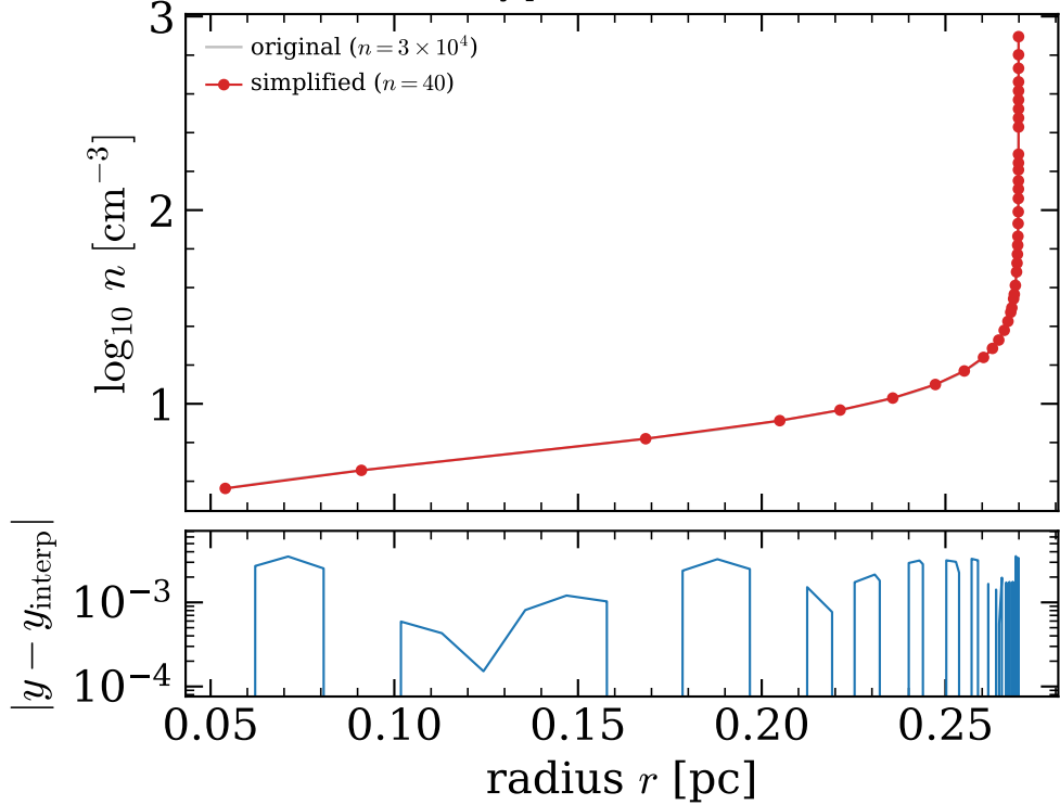
Density profile ( R^2 = 0.99999 )
