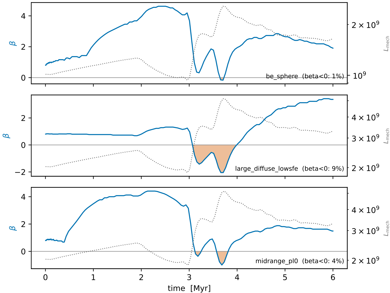
\beta(t) (red = \beta < 0 , P_b rising) vs mechanical luminosity
