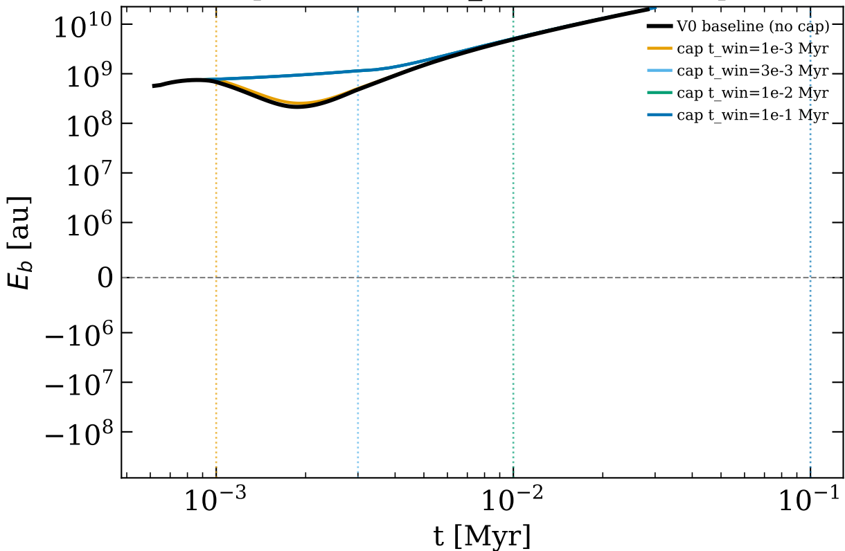
H4 PdV-cap: E_b(t) — mass_1e9 (dotted = cap release)
