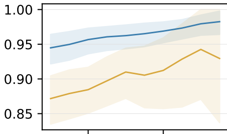
Accepted hit@3
