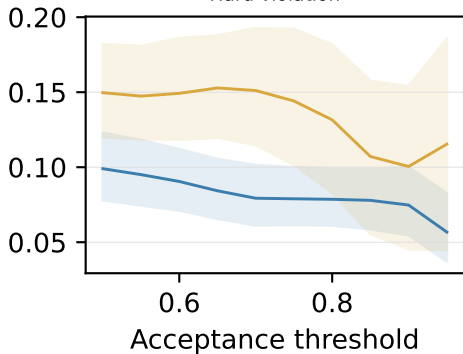
Hard violation
