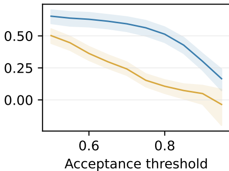
Net benefit
