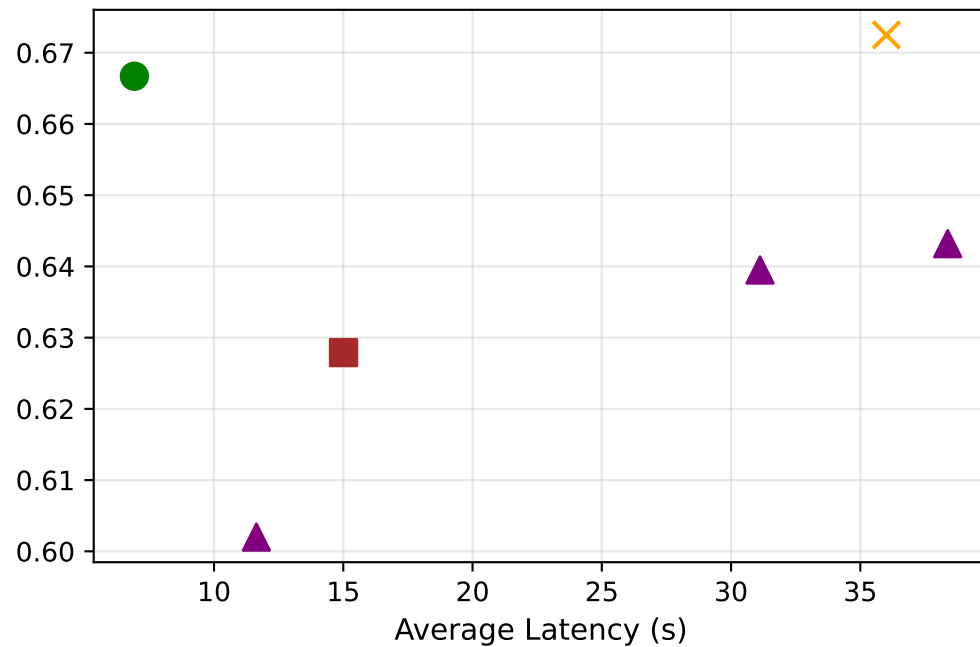
Task: Text-to-Visualization
