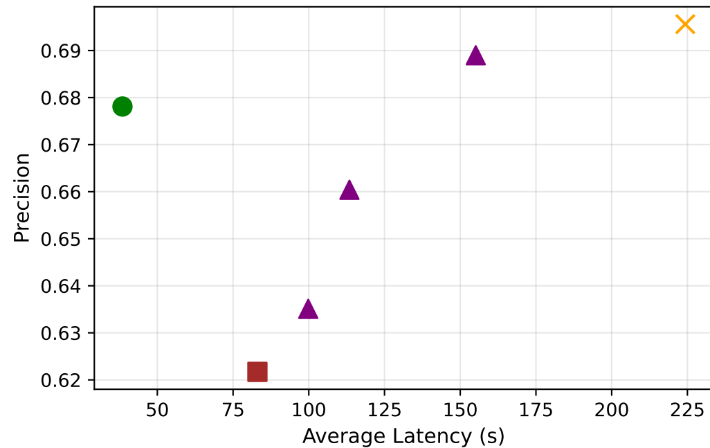
Task: Text-to-SQL
