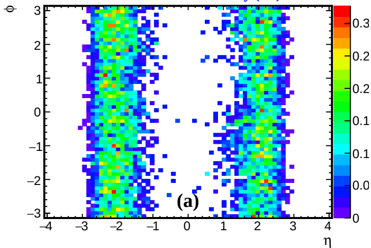
Reconstructed Efficiency ( K^+ )
