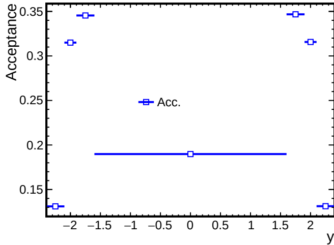
Coherent J/\psi (0n0n)
