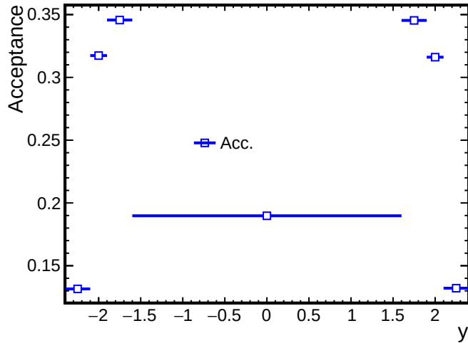
Coherent J/\psi (0nXn)
