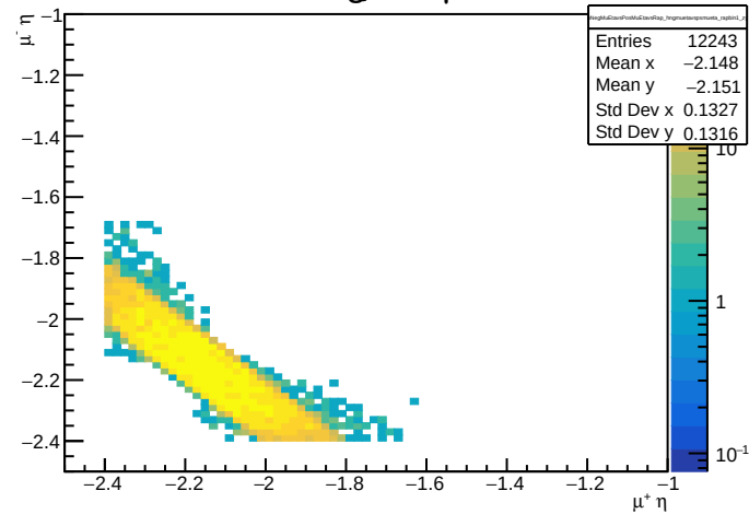
Daughter \mu
