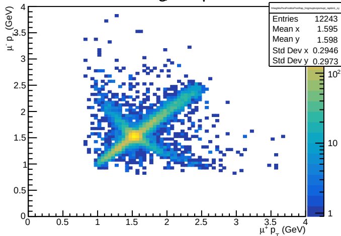
Daughter \mu
