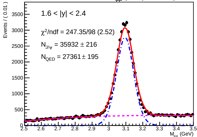
SA RooPlot of M_{\mu\mu} (GeV) 0.01840
