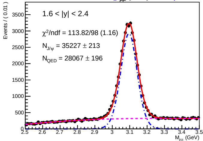
SA Root Plot of M_{\mu\mu} (GeV) 01420)
