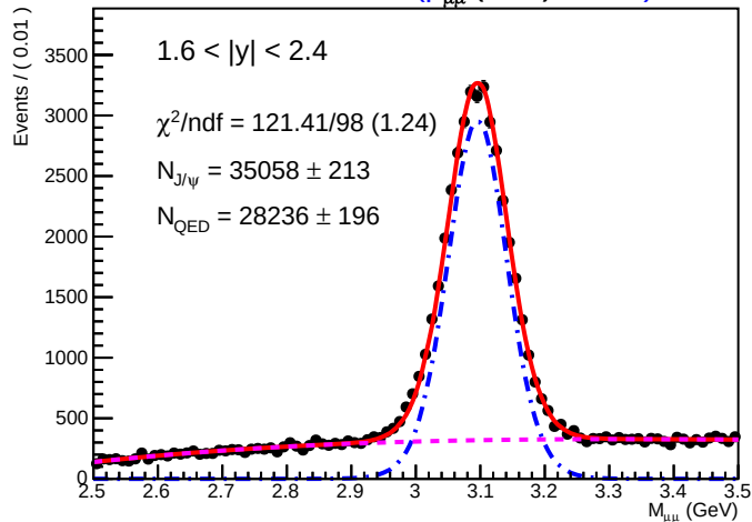
SA-RooPlot of M_{\mu\mu} (GeV) 01315
