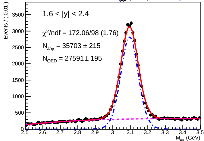
SA RooPlot of M_{\mu\mu} (GeV) 0.01705
