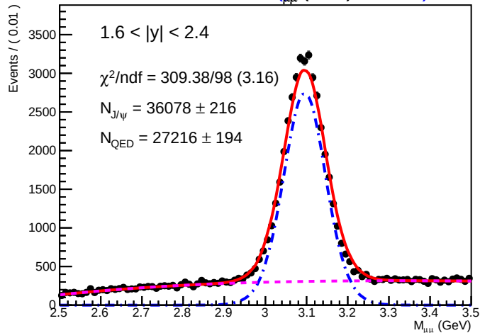
SA Root Plot of M_{\mu\mu} (GeV) 0.01925)
