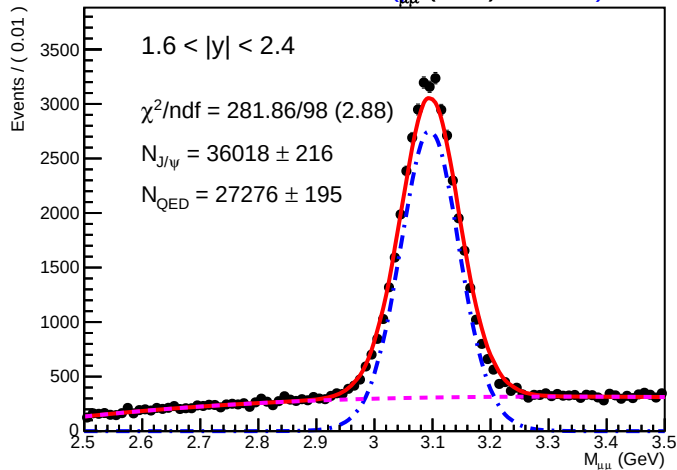
SA RooPlot of M_{\mu\mu} (GeV) 0.01890
