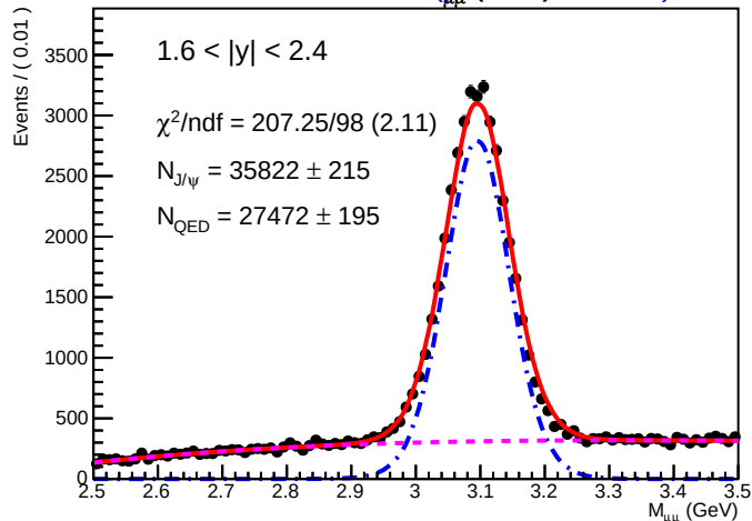
SA RooPlot of 5M μμ (GeV) 0.01775
