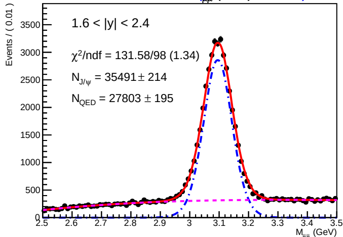
SA RooPlot of 6 M μμ (GeV) (0.01580)
