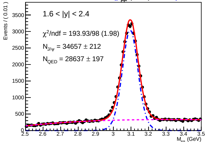
SA-RooPlot of M_{\mu\mu} (GeV) 1050
