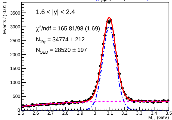
SA Root Plot of M_{\mu\mu} (GeV) 01130)
