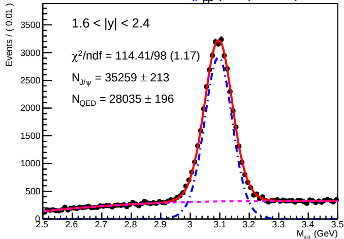
SA Root Plot of M_{\mu\mu} (GeV) 01440)
