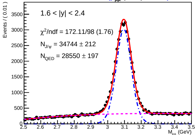
SA Root Plot of 'M μμ (GeV)' 01110)
