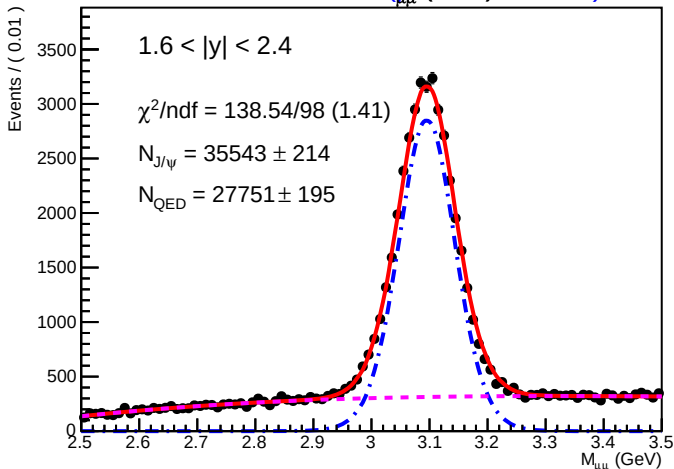
SA RooPlot of M_{\mu\mu}(\text{GeV}) .01610
