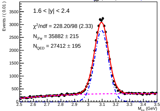
SA Root Plot of M_{\mu\mu} (GeV) 0.01810
