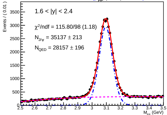
SA-RooPlot of M_{\mu\mu} (GeV) 01365
