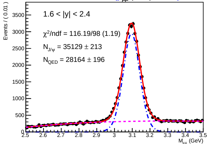
SA-RooPlot of M_{\mu\mu} (GeV) 01360
