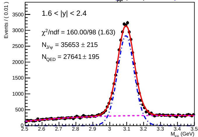
SA RooPlot of 5 M μμ (GeV) (0.1675)
