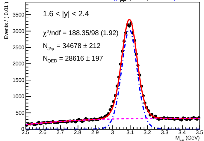
SA Root Plot of M_{\mu\mu} (GeV) 01065
