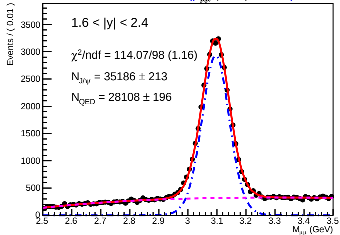
SAARD Plot of M_{\mu\mu} (GeV) 01395
