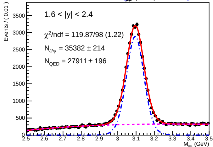
SA RooPlot of M_{\mu\mu}(\text{GeV}) .01515
