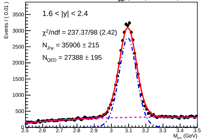
SA Root Plot of M_{\mu\mu} (GeV) 0.01825
