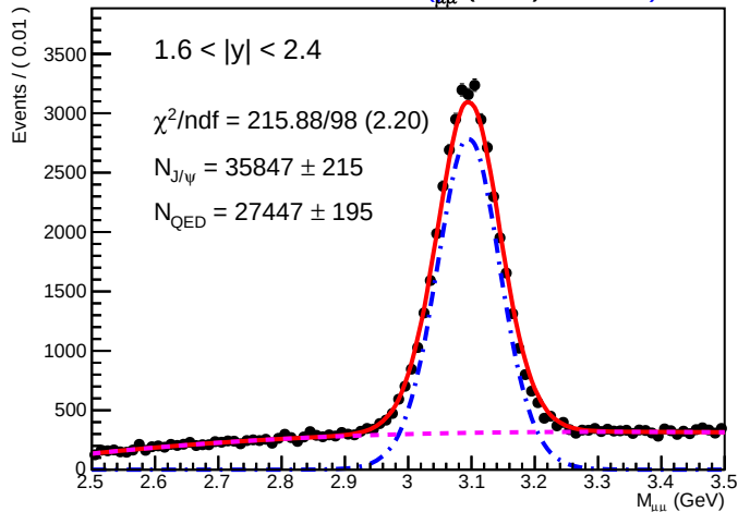
SA RooPlot of M_{\mu\mu}(\text{GeV}) .01790
