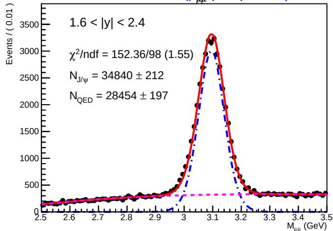
SA Root Plot of M_{\mu\mu} (GeV) 01175)
