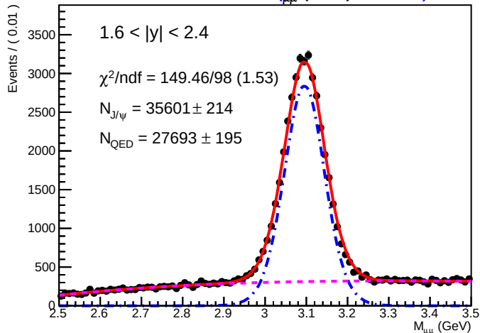
SA RooPlot of M_{\mu\mu} (GeV) 0.01645
