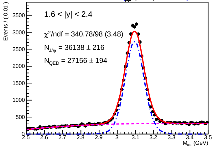
SA Root Plot of 2 M μμ (GeV) 2 .01960)
