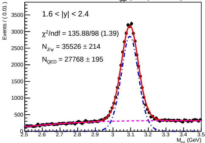
SA RooPlot of M_{\mu\mu}(\text{GeV}) .01600
