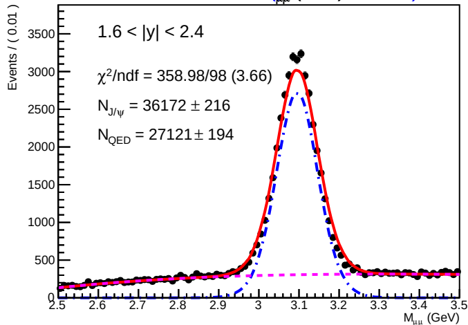
SA RooPlot of M_{\mu\mu} (GeV) 0.01980
