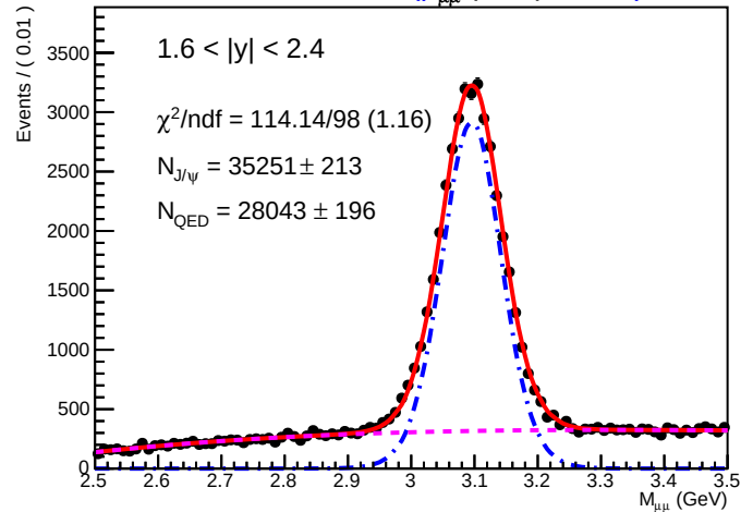
SA Root Plot of M_{\mu\mu} (GeV) 01435)
