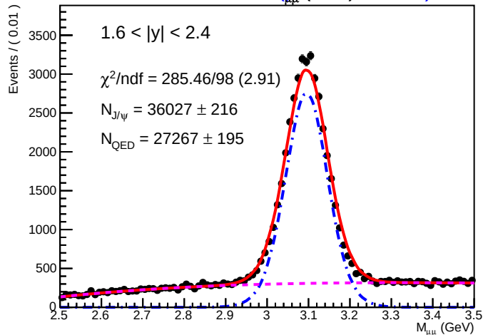
SA RooPlot of M_{\mu\mu} (GeV) 0.01895
