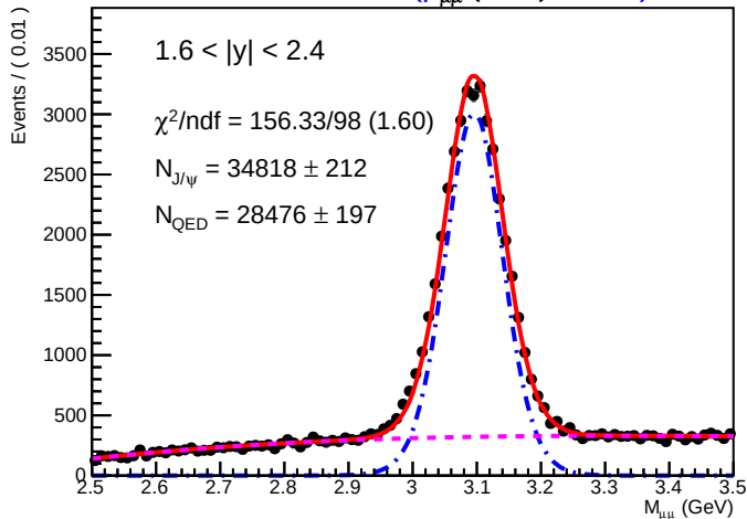
SA Root Plot of M_{\mu\mu} (GeV) 01160)
