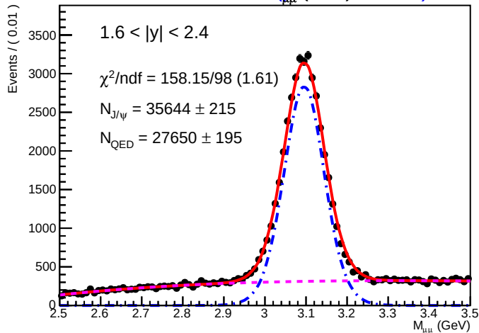
SA RooPlot of 4 M μμ (GeV) (0.1670)
