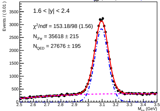
SA RooPlot of M_{\mu\mu} (GeV) 0.01655
