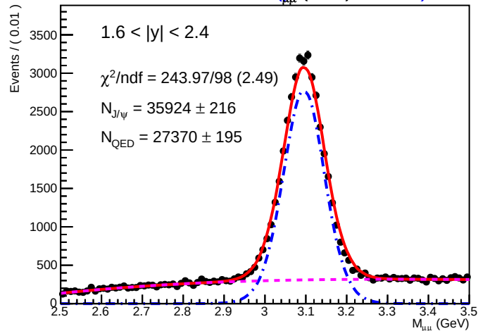
SA Root Plot of M_{\mu\mu} (GeV) 0.01835
