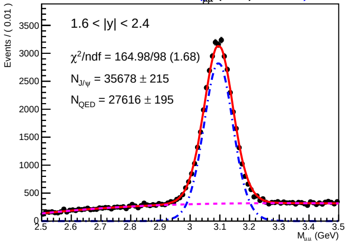
SA RooPlot of M_{\mu\mu}(\text{GeV}) .01690
