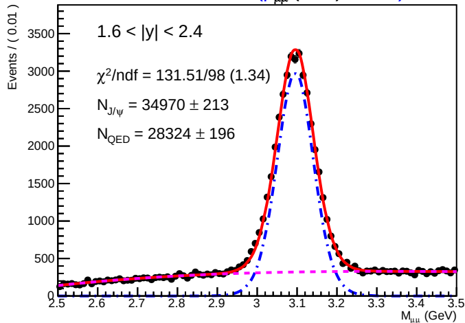
SA Root Plot of M_{\mu\mu} (GeV) 01260)
