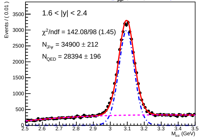
SA Root Plot of M_{\mu\mu} (GeV) 01215)
