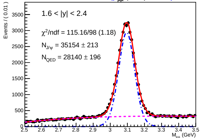
SA-RooPlot of M_{\mu\mu} (GeV) 01375
