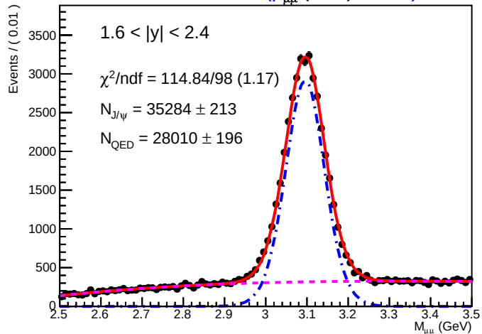
SA Root Plot of M_{\mu\mu} (GeV) 01455)
