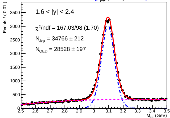
SA Root Plot of M_{\mu\mu} (GeV) 01125)
