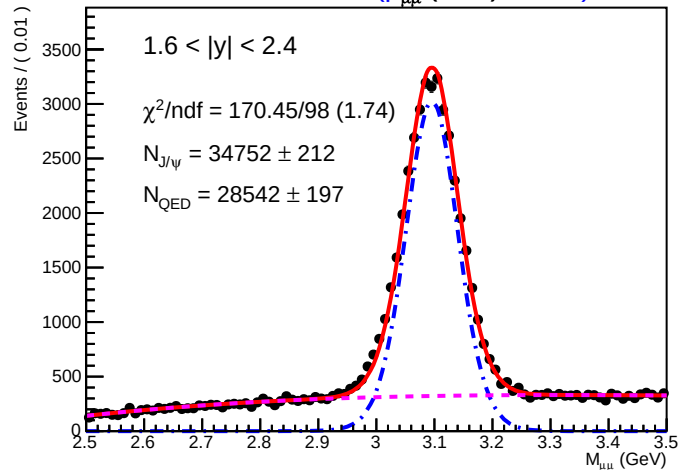
SA Root Plot of 'M μμ (GeV)' 01115)
