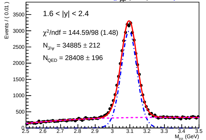
SA Root Plot of M_{\mu\mu} (GeV) 01205)
