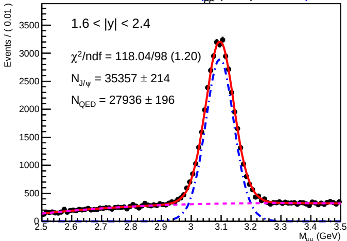
SA RooPlot of M_{\mu\mu}(\text{GeV}) .01500
