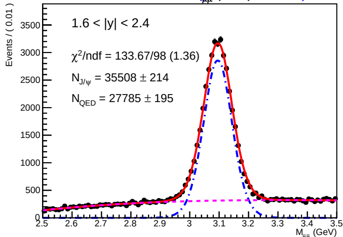
SA RooPlot of 8 M μμ (GeV) (0.01590)
