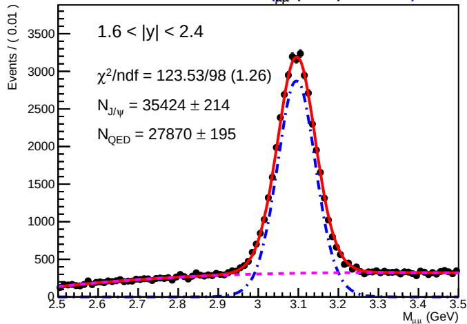
SA RooPlot of M_{\mu\mu} (GeV) 0.01540
