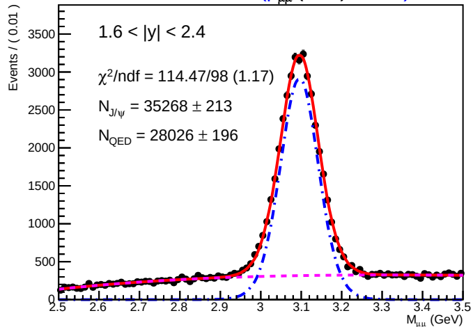
SA Root Plot of M_{\mu\mu} (GeV) 01445)
