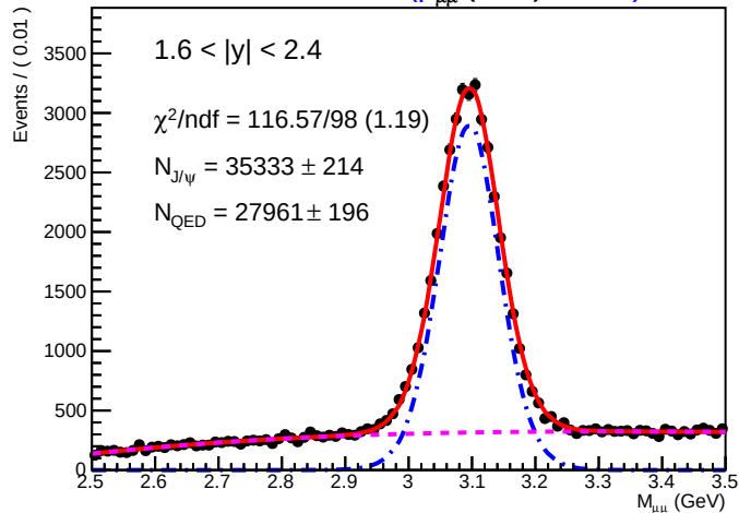
SA-RooPlot of M_{\mu\mu} (GeV) 01485
