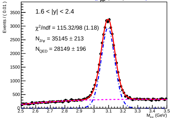
SA-RooPlot of M_{\mu\mu} (GeV) 01370
