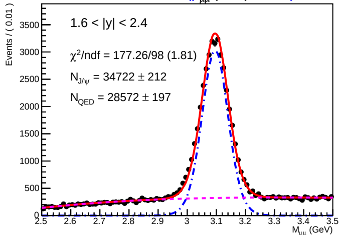
SA-RooPlot of M_{\mu\mu} (GeV) 01095
