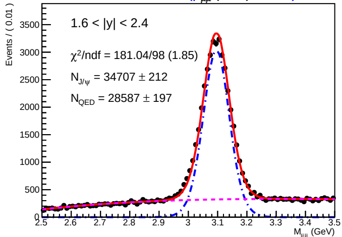
SA-RooPlot of M_{\mu\mu} (GeV) 01085
