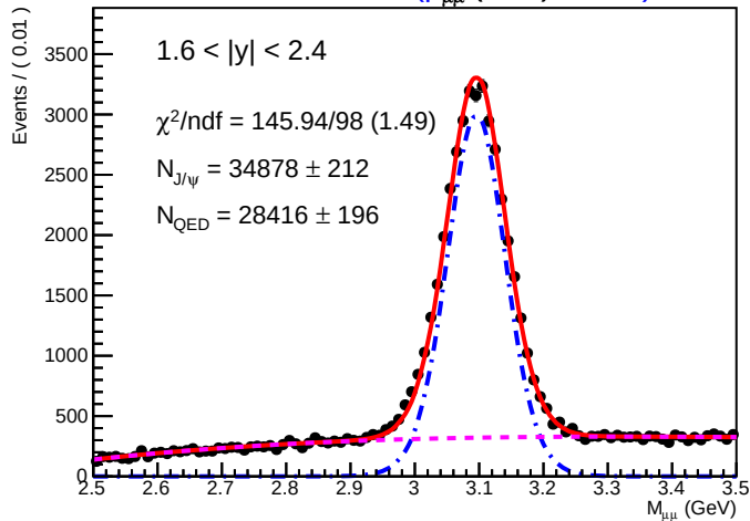
SA Root Plot of M_{\mu\mu} (GeV) 01200)
