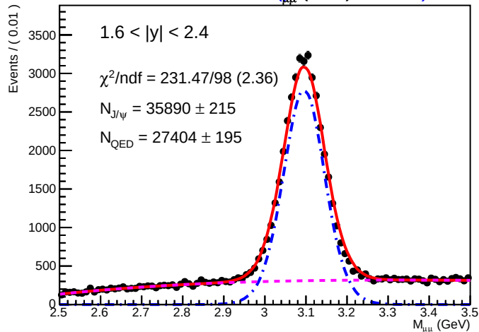
SA Root Plot of M_{\mu\mu} (GeV) 0.01815
