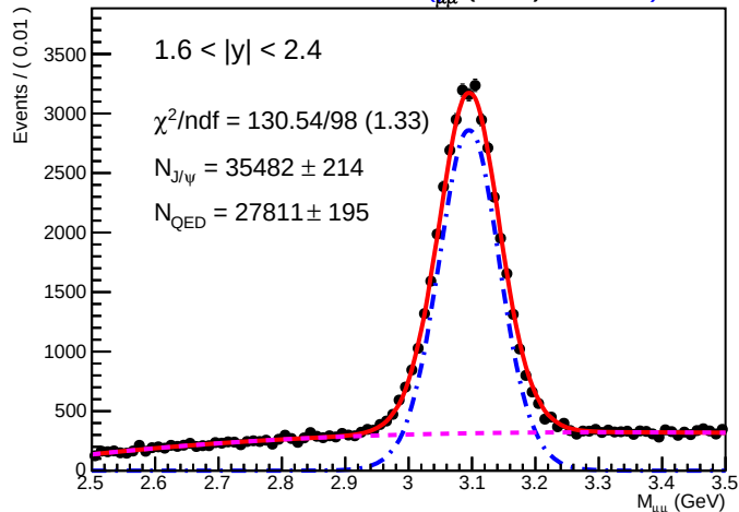
SA RooPlot of 5 M μμ (GeV) (0.01575)
