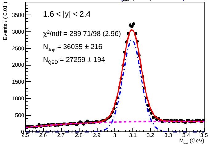
SA Root Plot of M_{\mu\mu} (GeV)
