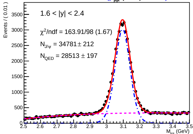
SA Root Plot of M_{\mu\mu} (GeV) 01135)
