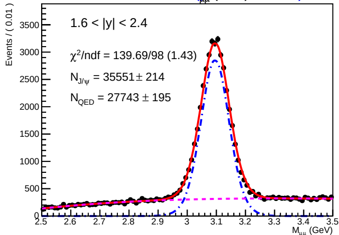
SA RooPlot of M_{\mu\mu}(\text{GeV}) .01615
