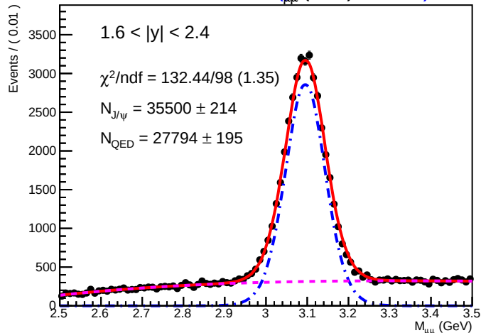
SA RooPlot of 7 M μμ (GeV) (0.01585)
