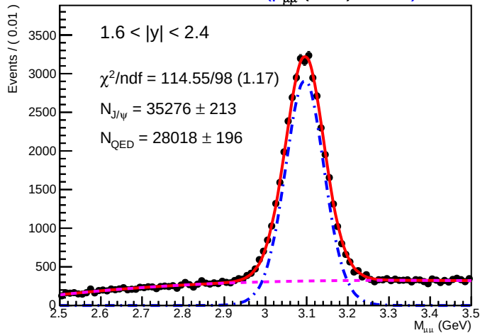
SA Root Plot of M_{\mu\mu} (GeV) 01450)
