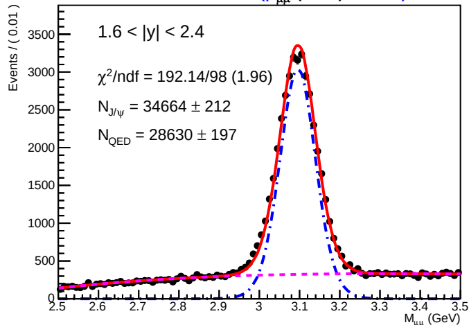
SA-RooPlot of M_{\mu\mu} (GeV) 1055
