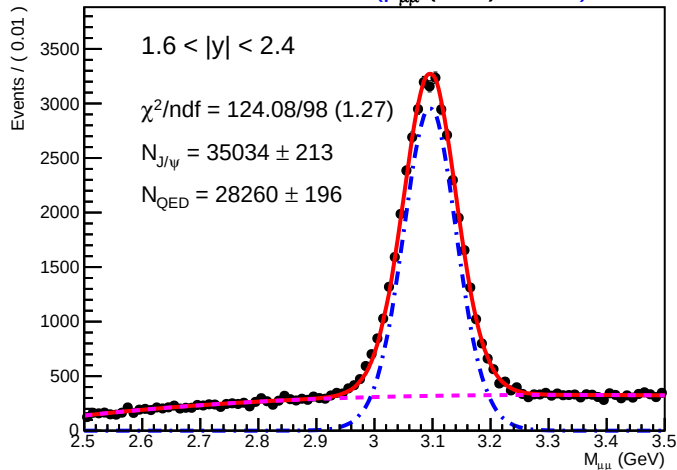
SA-RooPlot of M_{\mu\mu} (GeV) 01300
