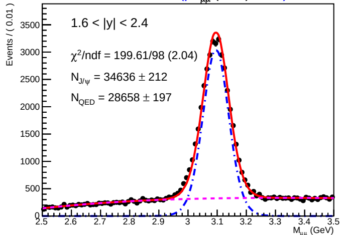
SA Root Plot of M_{\mu\mu} (GeV) 1035)
