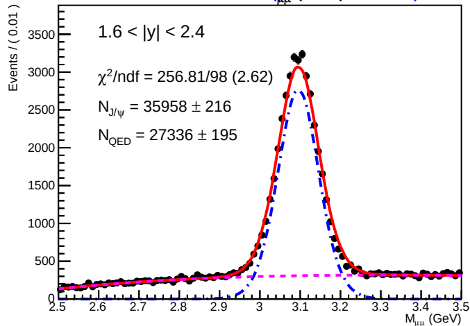
SA RooPlot of M_{\mu\mu} (GeV) 0.01855
