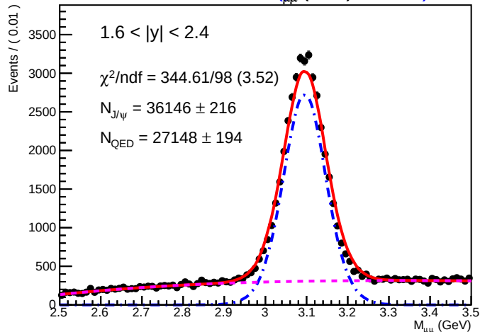
SA Root Plot of 3 M μμ (GeV) 3 .01965)
