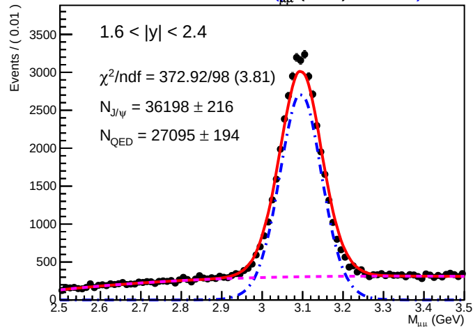
SA RooPlot of M_{\mu\mu} (GeV) 0.01995
