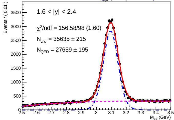
SA RooPlot of 3 M μμ (GeV) (0.1665)
