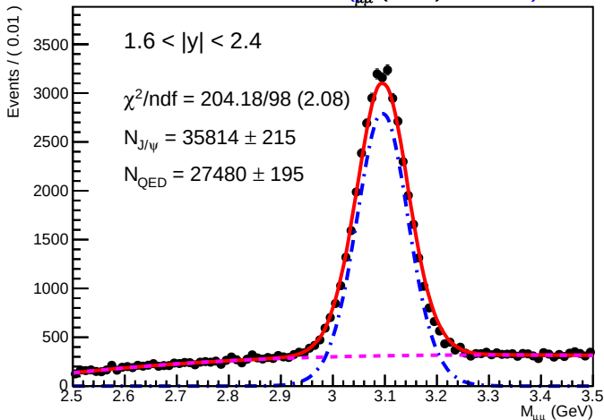
SA RooPlot of 4M μμ (GeV) 0.01770
