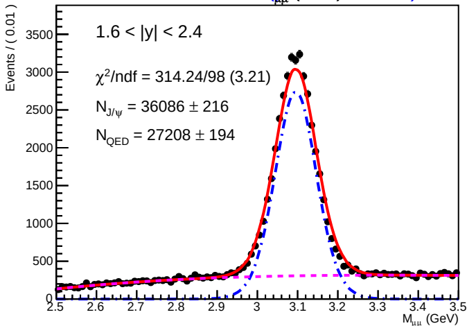
SA Root Plot of M_{\mu\mu} (GeV) 0.01930)
