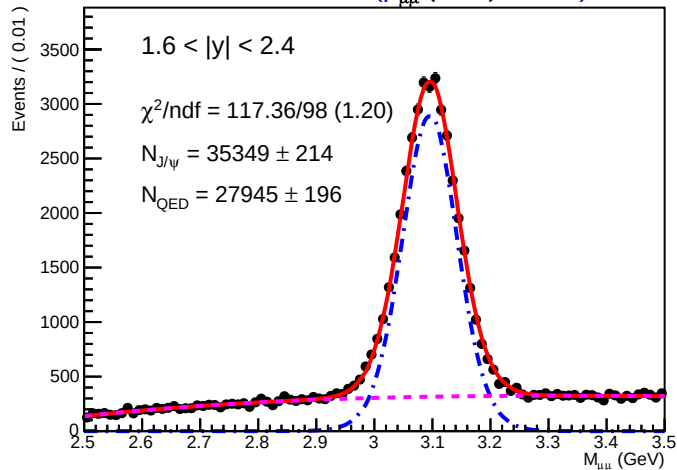
SA-RooPlot of M_{\mu\mu} (GeV) 01495
