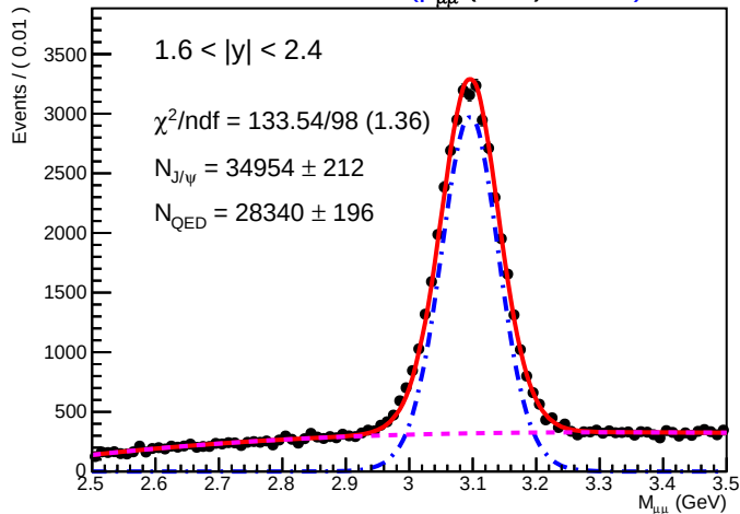
SA Root Plot of M_{\mu\mu} (GeV) 01250)
