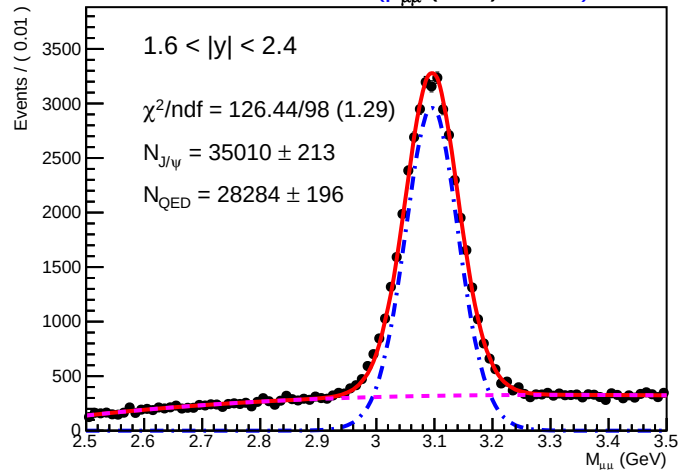
SA-RooPlot of M_{\mu\mu} (GeV) 01285
