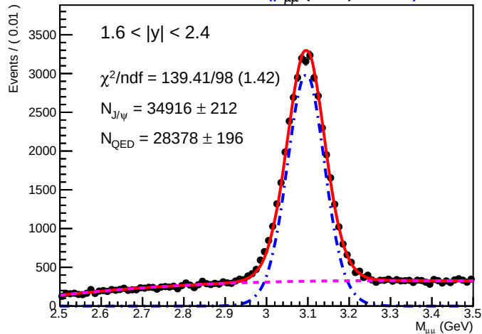
SA Root Plot of M_{\mu\mu} (GeV) 01225)
