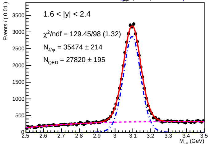
SA RooPlot of 4 M μμ (GeV) (0.01570)
