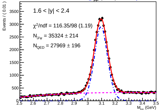
SA-RooPlot of M_{\mu\mu} (GeV) 01480
