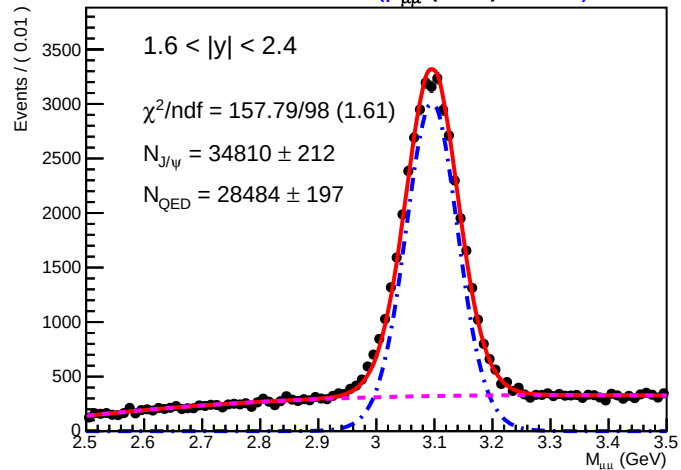
SA-RooPlot of M_{\mu\mu} (GeV) 01155)
