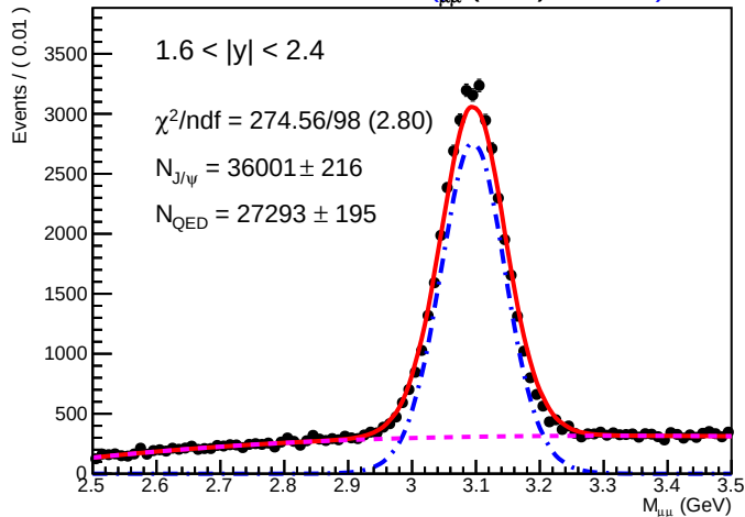
SA RooPlot of M_{\mu\mu} (GeV) 0.01880
