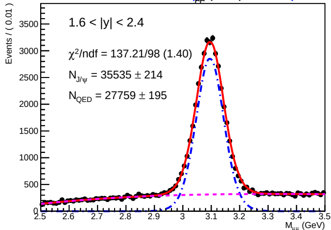
SA RooPlot of M_{\mu\mu}(\text{GeV}) .01605
