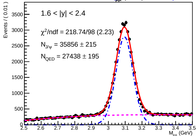
SA RooPlot of M_{\mu\mu}(\text{GeV}) .01795
