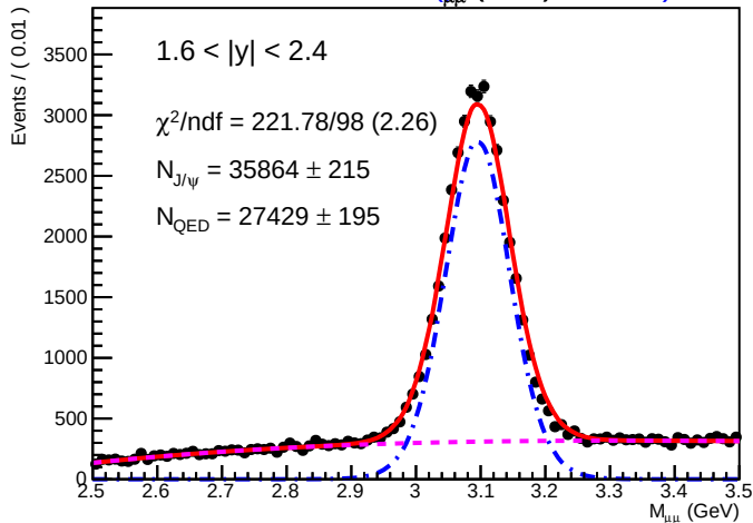
SA Root Plot of M_{\mu\mu} (GeV) 0.01800
