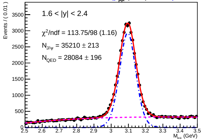
SA-RDPlot of M_{\mu\mu} (GeV) 01410
