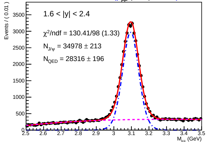
SA Root Plot of M_{\mu\mu} (GeV) 01265)
