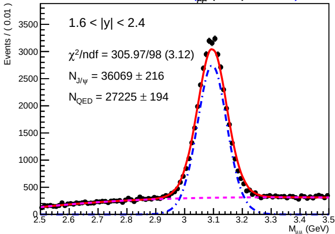
SA Root Plot of M_{\mu\mu} (GeV) 0.01920)
