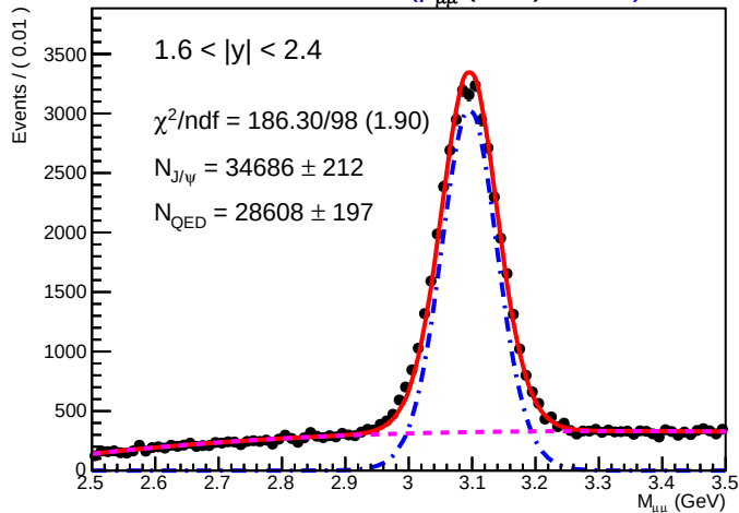
SA Root Plot of M_{\mu\mu} (GeV) 01070
