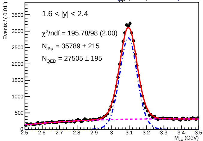
SA RooPlot of M_{\mu\mu} (GeV) 0.01755
