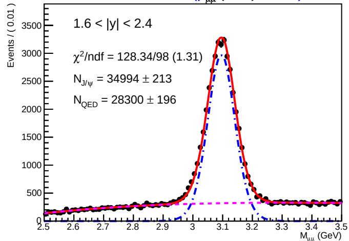
SA Root Plot of M_{\mu\mu} (GeV) 01275)
