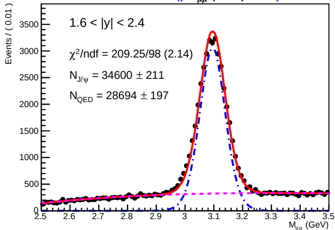
SA RooPlot of (M_{\mu\mu}) (GeV)
