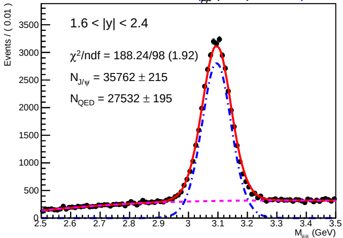
SA RooPlot of M_{\mu\mu} (GeV) 0.01740
