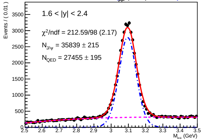
SA RooPlot of M_{\mu\mu}(\text{GeV}) .01785
