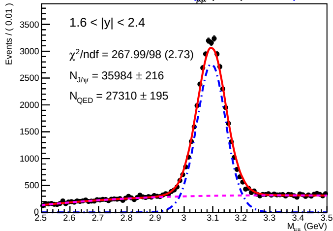
SA RooPlot of 4M μμ (GeV) (0.1870)
