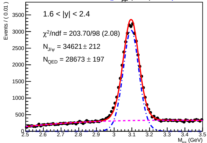
SA Root Plot of M_{\mu\mu} (GeV) 1025)
