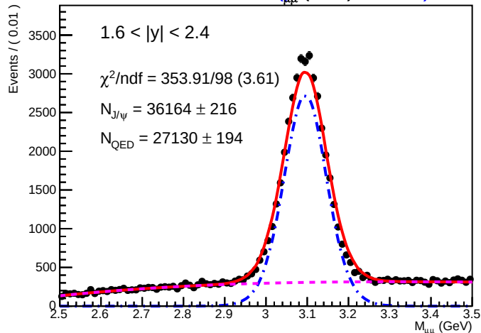
SA Root Plot of 5 M μμ (GeV) 5 .01975)
