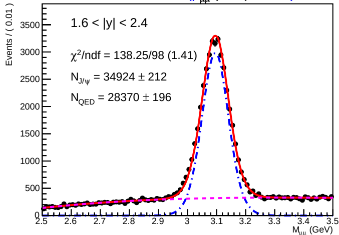
SA Root Plot of M_{\mu\mu} (GeV) 01230)
