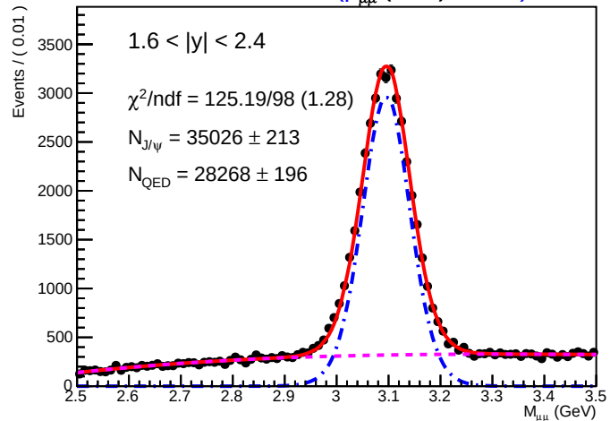
SA-RooPlot of M_{\mu\mu} (GeV) 01295
