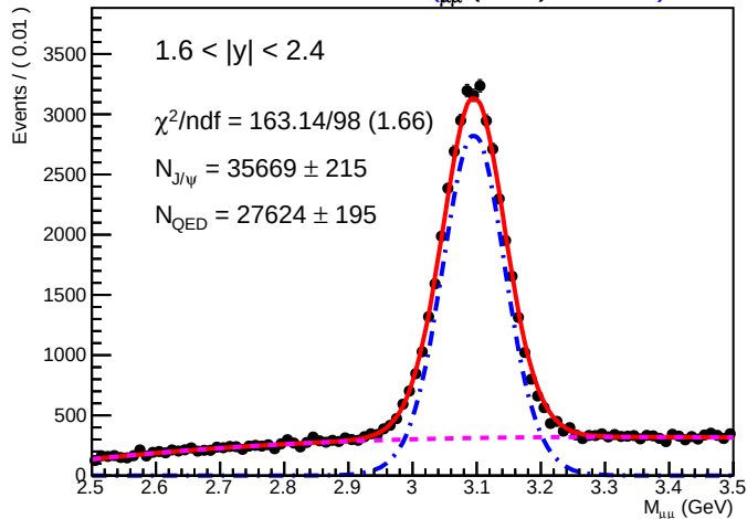
SA RooPlot of M_{\mu\mu}(\text{GeV}) .01685
