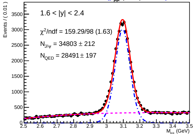
SA-RooPlot of M_{\mu\mu} (GeV) 01150)
