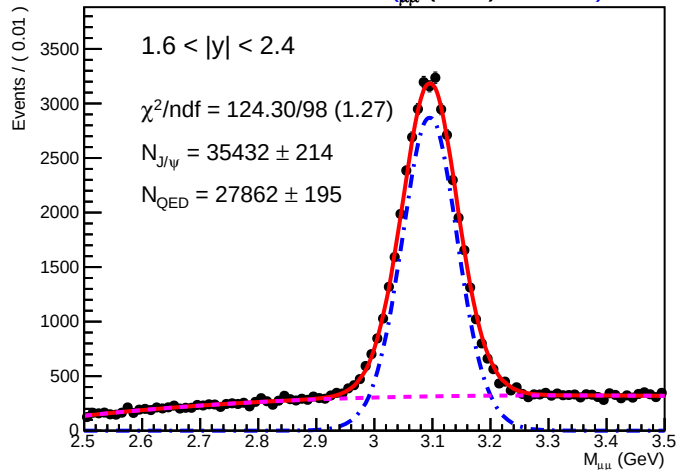
SA RooPlot of M_{\mu\mu} (GeV) 0.01545
