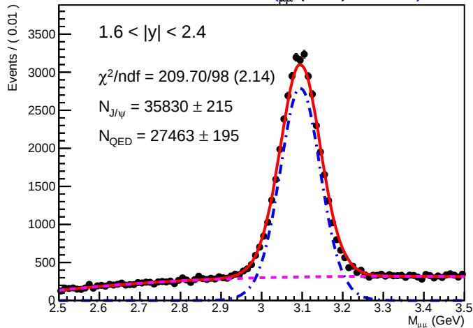
SA RooPlot of M_{\mu\mu}(\text{GeV}) .01780
