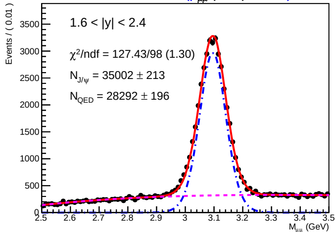
SA-RooPlot of M_{\mu\mu} (GeV) 01280
