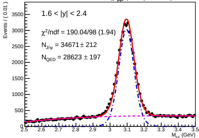
SA Root Plot of M_{\mu\mu} (GeV) 01060
