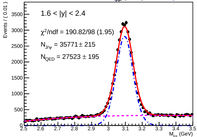
SA RooPlot of M_{\mu\mu} (GeV) 0.01745
