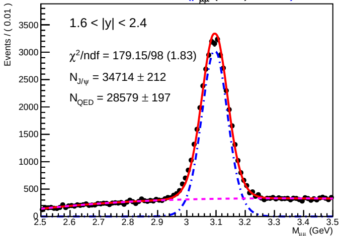
SA-RooPlot of M_{\mu\mu} (GeV) 01090
