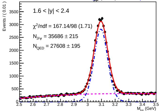
SA RooPlot of M_{\mu\mu}(\text{GeV}) .01695
