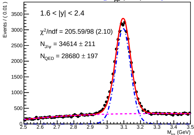
SA Root Plot of M_{\mu\mu} (GeV) 1020)
