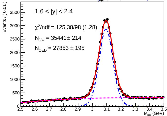
SA RooPlot of M_{\mu\mu} (GeV) 0.01550
