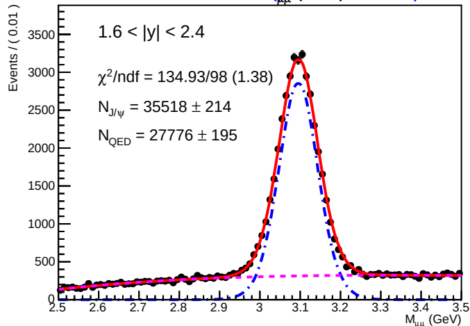
SA RooPlot of 9 M μμ (GeV) (0.01595)
