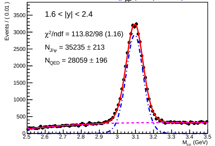
SA Root Plot of M_{\mu\mu} (GeV) 01425)
