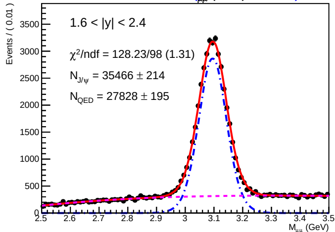
SA RooPlot of 3 M μμ (GeV) (0.01565)
