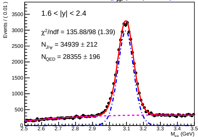
SA Root Plot of M_{\mu\mu} (GeV) 01240)
