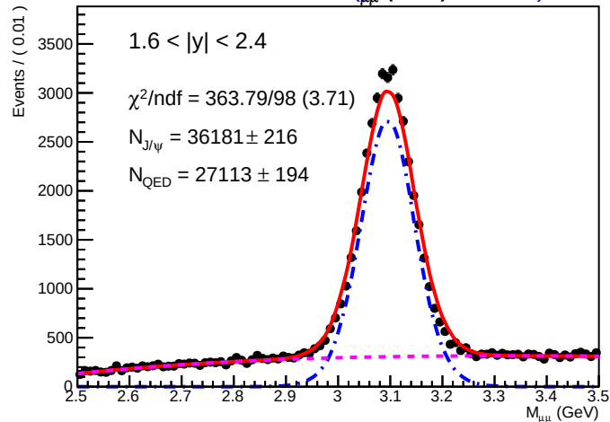
SA RooPlot of M_{\mu\mu} (GeV) 0.01985
