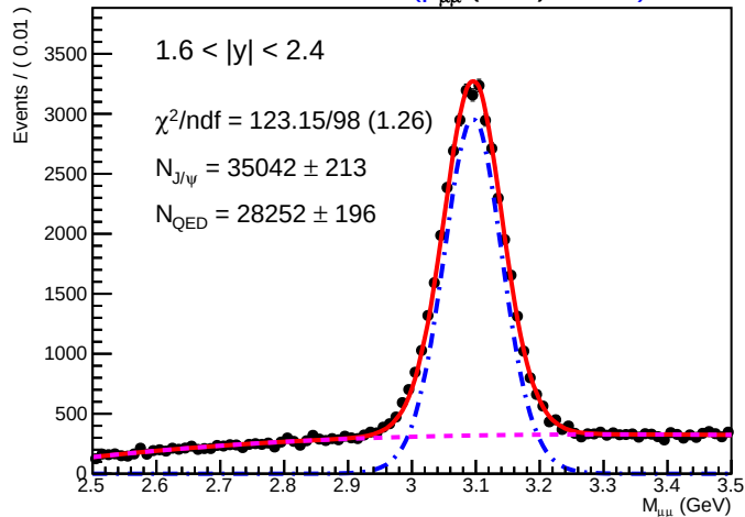
SA-RooPlot of M_{\mu\mu} (GeV) 01305
