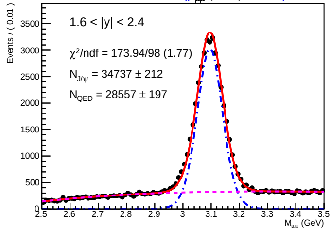
SA Root Plot of 'M μμ (GeV)' 01105)
