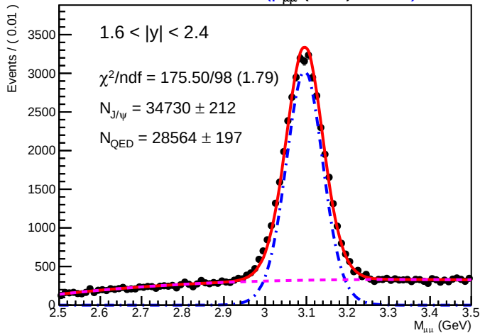
SA Root Plot of 'M μμ (GeV)' 01100)
