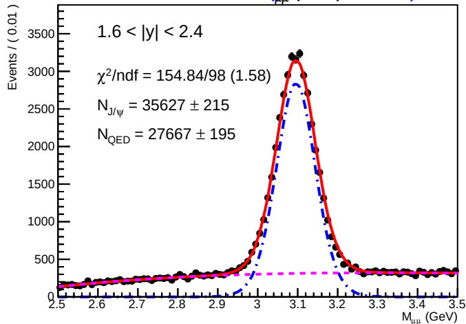
SA RooPlot of 2 M μμ (GeV) (0.1660)
