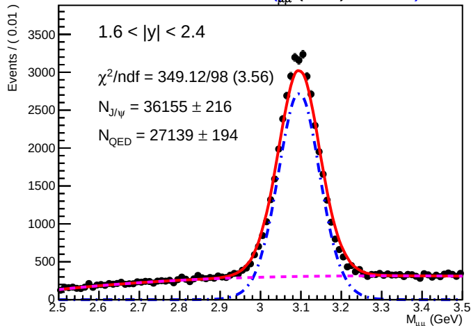
SA Root Plot of 4 M μμ (GeV) 4 .01970)
