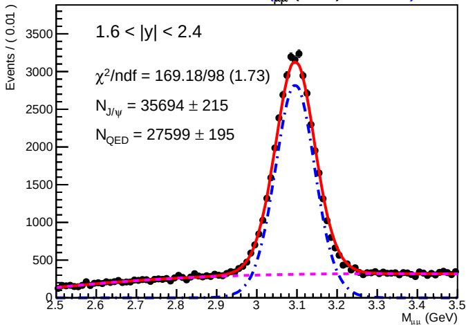
SA RooPlot of M_{\mu\mu} (GeV) 0.01700
