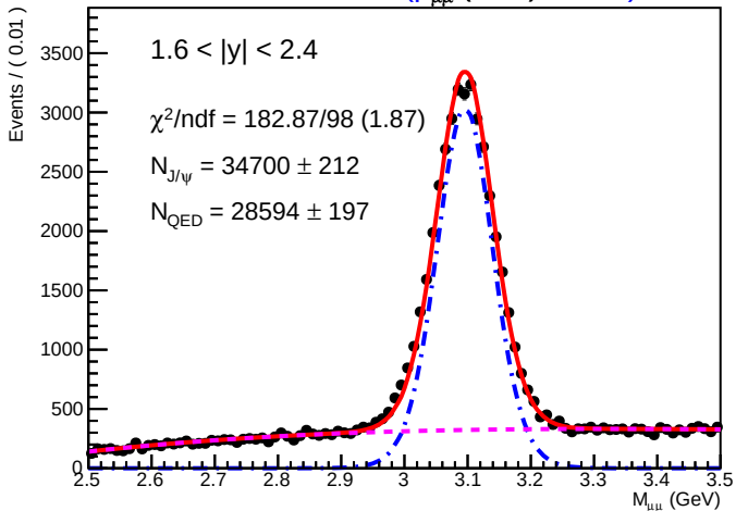
SA-RooPlot of M_{\mu\mu} (GeV) 01080
