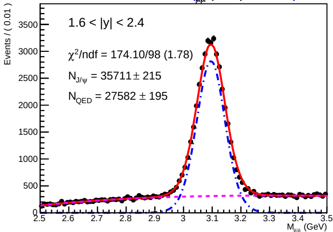
SA RooPlot of M_{\mu\mu} (GeV) 0.01710
