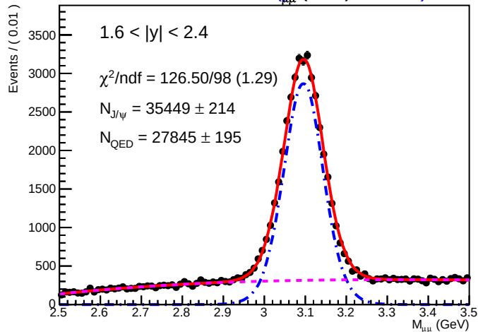
SA RooPlot of M_{\mu\mu} (GeV) 0.01555
