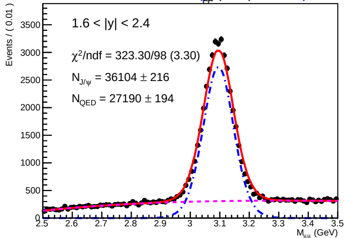
SA RooPlot of M_{\mu\mu} (GeV) 0.01940
