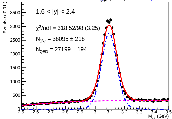
SA Root Plot of M_{\mu\mu} (GeV) 0.01935)
