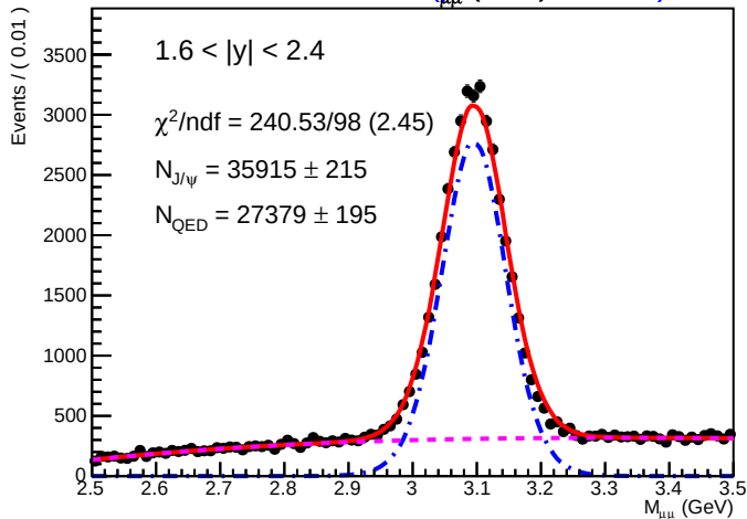
SA Root Plot of M_{\mu\mu} (GeV) 0.01830
