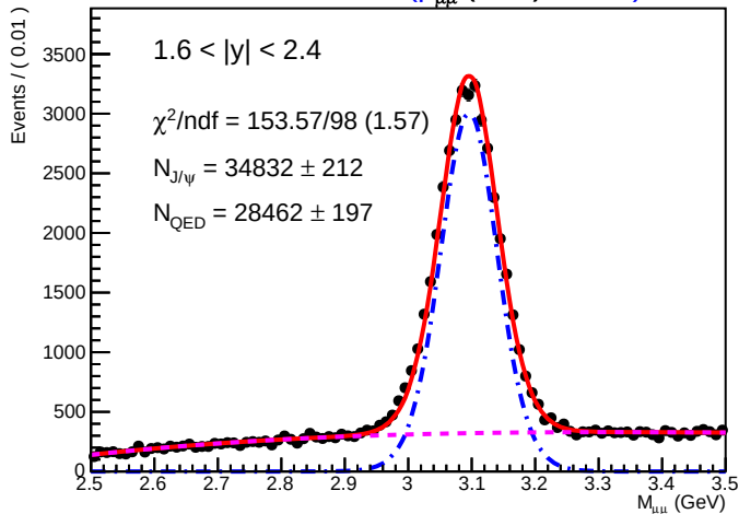
SA Root Plot of M_{\mu\mu} (GeV) 01170)
