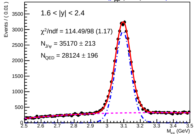
SAARD Plot of M_{\mu\mu} (GeV) 01385
