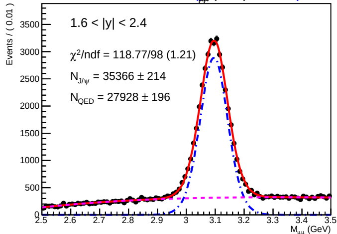
SA RooPlot of M_{\mu\mu}(\text{GeV}) .01505
