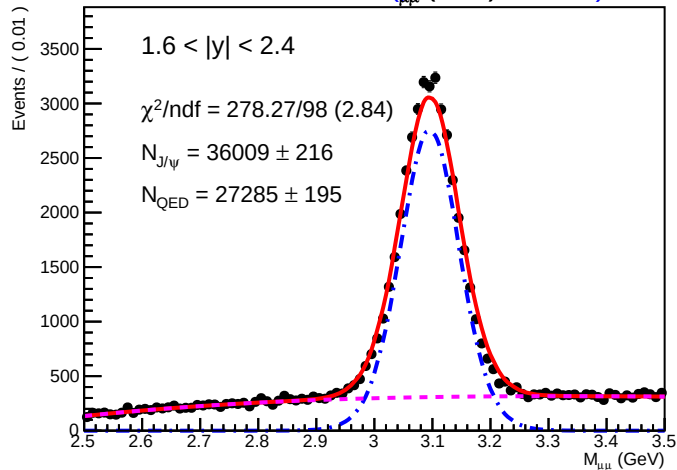
SA RooPlot of M_{\mu\mu} (GeV) 0.01885
