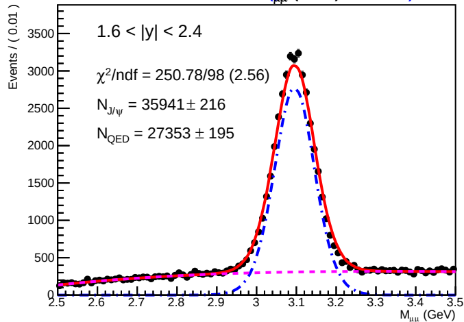
SA RooPlot of M_{\mu\mu} (GeV) 0.01845
