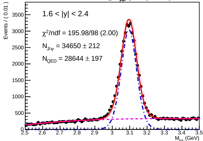
SA-RooPlot of M_{\mu\mu} (GeV) 1045
