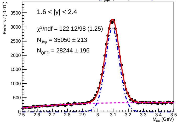
SA-RooPlot of M_{\mu\mu} (GeV) 01310
