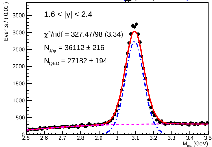
SA RooPlot of M_{\mu\mu} (GeV) 0.01945
