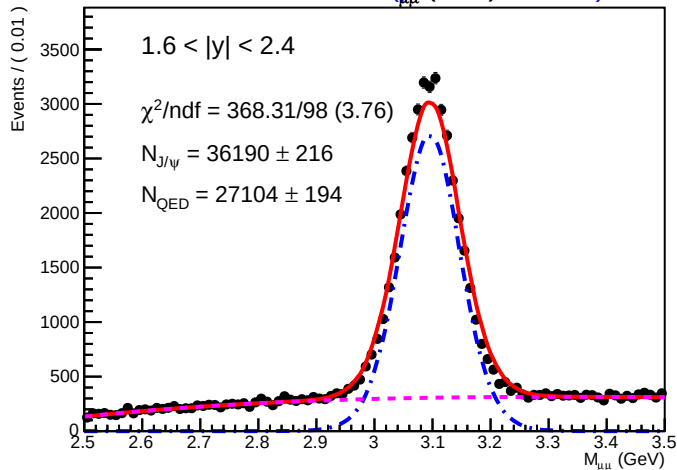
SA RooPlot of M_{\mu\mu} (GeV) 0.01990
