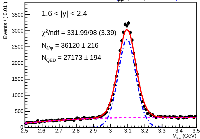
SA RooPlot of M_{\mu\mu} (GeV) 0.01950
