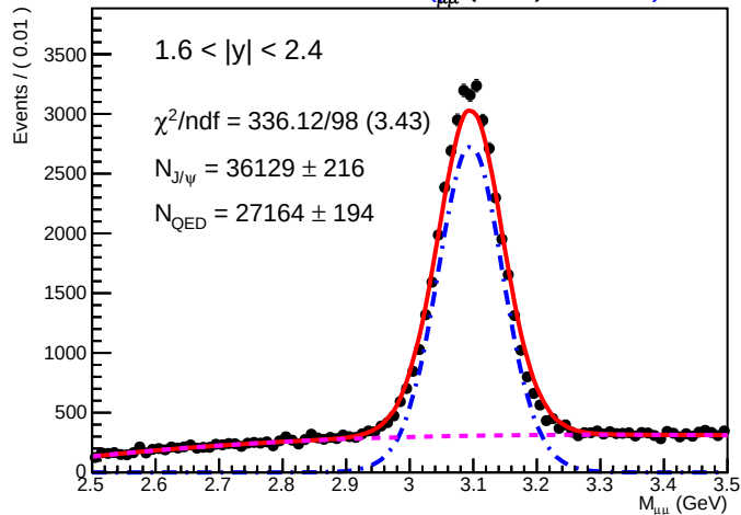
SA RooPlot of M_{\mu\mu} (GeV) 0.01955
