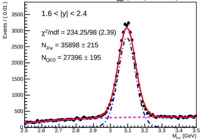
SA Root Plot of M_{\mu\mu} (GeV) 0.01820
