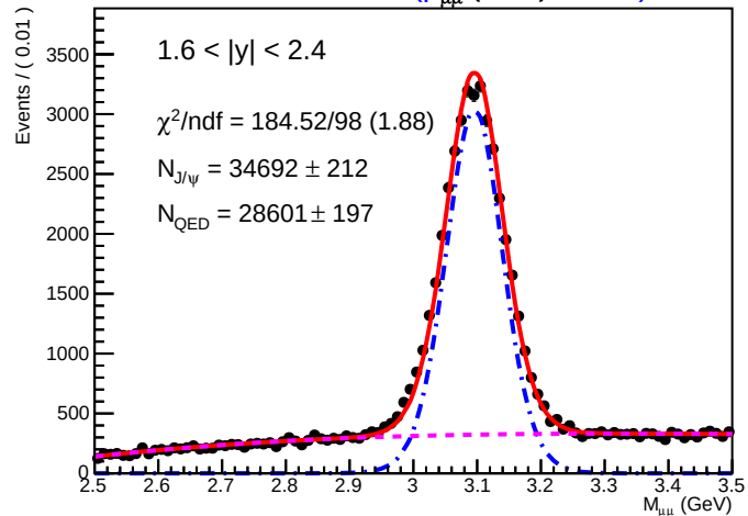
SA Root Plot of M_{\mu\mu} (GeV) 01075
