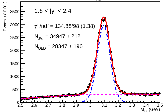
SA Root Plot of M_{\mu\mu} (GeV) 01245)
