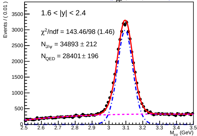
SA Root Plot of M_{\mu\mu} (GeV) 01210)
