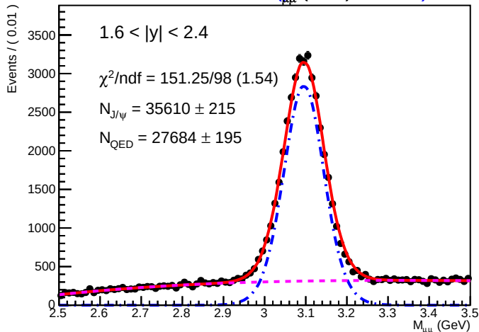
SA RooPlot of M_{\mu\mu} (GeV) 0.01650
