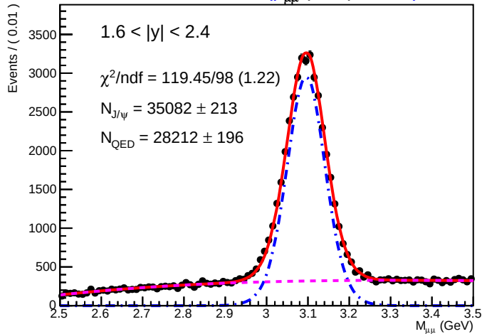
SA-RooPlot of M_{\mu\mu} (GeV) 01330)
