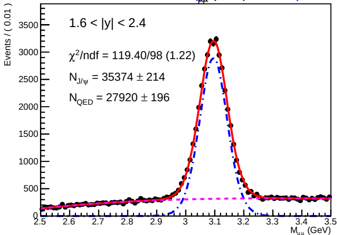
SA RooPlot of M_{\mu\mu}(\text{GeV}) .01510
