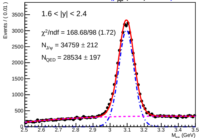
SA Root Plot of M_{\mu\mu} (GeV) 01120)
