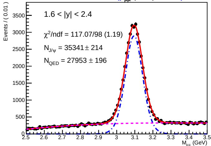
SA-RooPlot of M_{\mu\mu} (GeV) 01490
