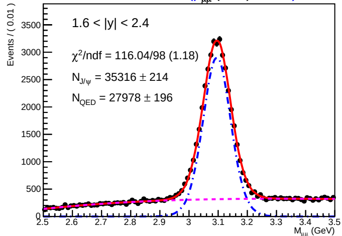
SA-RooPlot of M_{\mu\mu} (GeV) 01475)
