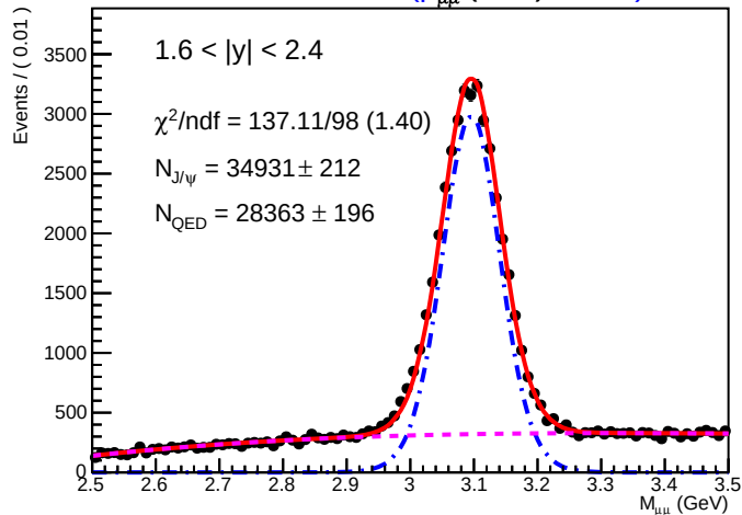
SA Root Plot of M_{\mu\mu} (GeV) 01235)
