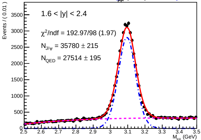
SA RooPlot of M_{\mu\mu} (GeV) 0.01750
