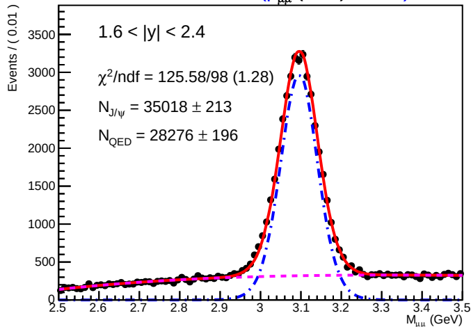
SA-RooPlot of M_{\mu\mu} (GeV) 01290
