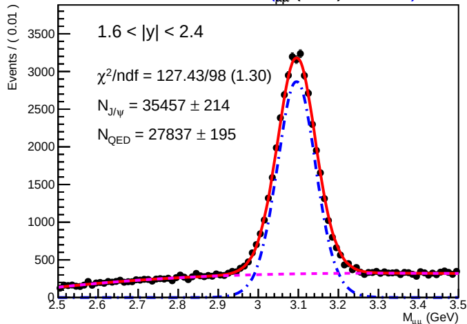
SA RooPlot of 2 M μμ (GeV) (0.01560)
