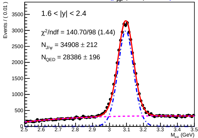
SA Root Plot of M_{\mu\mu} (GeV) 01220)
