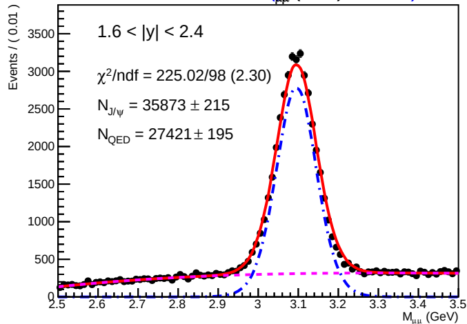
SA Root Plot of M_{\mu\mu} (GeV) 0.01805
