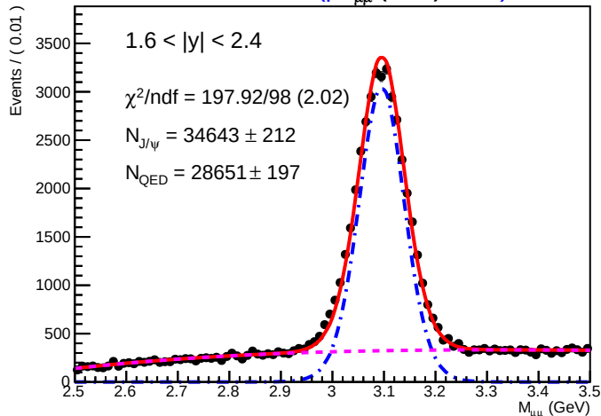
SA-RooPlot of M_{\mu\mu} (GeV) 1040
