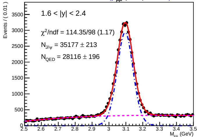
SAARD Plot of M_{\mu\mu} (GeV) 01390
