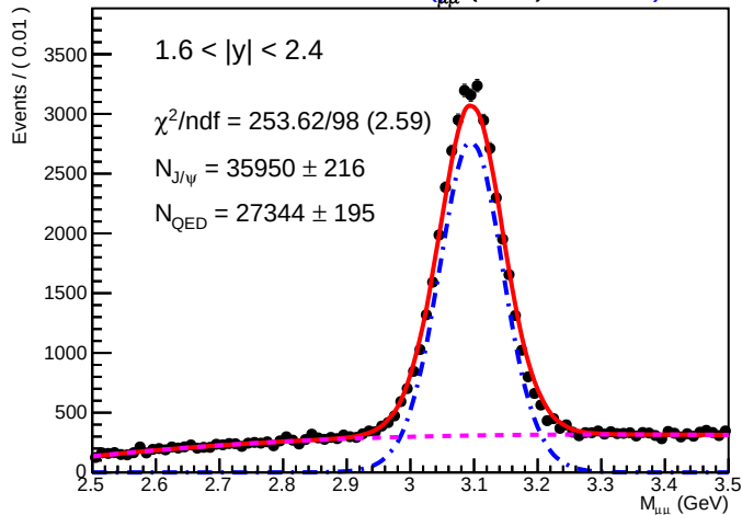
SA RooPlot of M_{\mu\mu} (GeV) 0.01850
