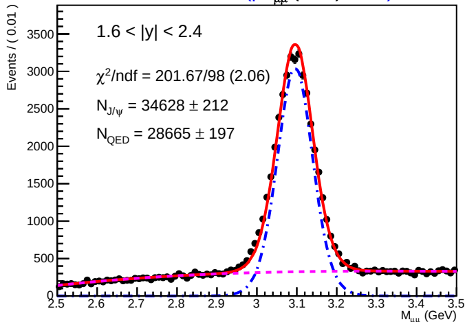
SA Root Plot of M_{\mu\mu} (GeV) 1030)
