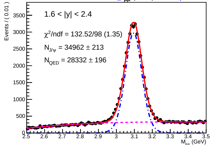
SA Root Plot of M_{\mu\mu} (GeV) 01255)
