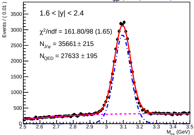
SA RooPlot of M_{\mu\mu}(\text{GeV}) .01680
