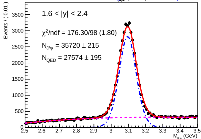
SA RooPlot of M_{\mu\mu} (GeV) 0.01715
