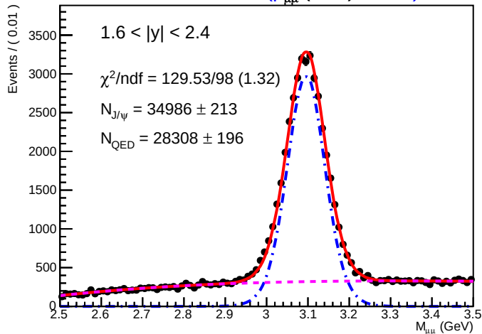
SA Root Plot of M_{\mu\mu} (GeV) 01270)
