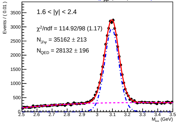
SAARD Plot of M_{\mu\mu} (GeV) 01380
