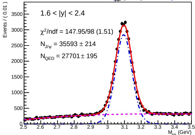
SA RooPlot of M_{\mu\mu} (GeV) 0.01640
