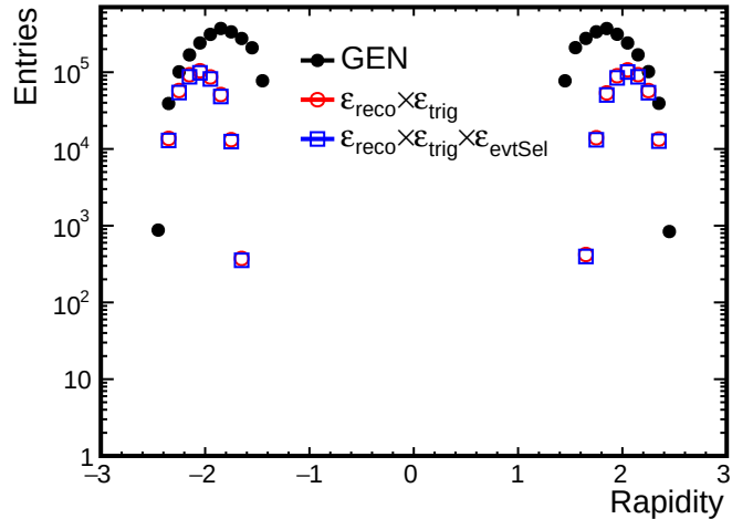
Coh. J/\psi (0nXn)
