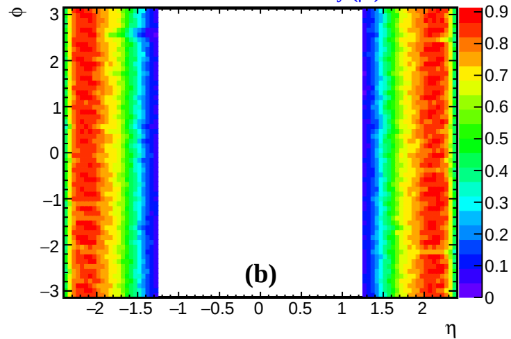
Reconstructed Efficiency ( \mu^- )
