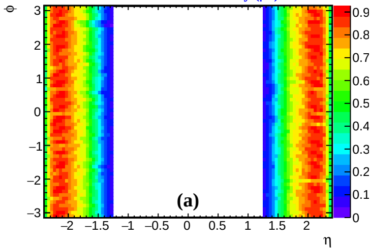
Reconstructed Efficiency ( \mu^+ )
