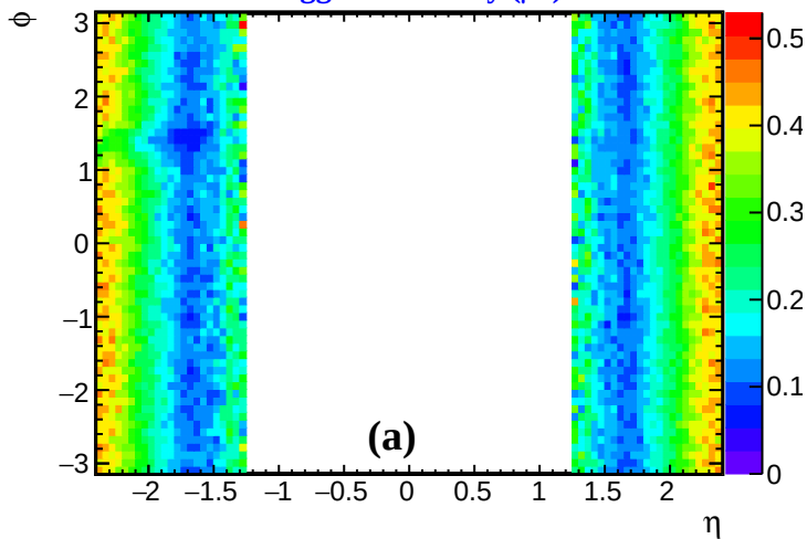
Trigger Efficiency ( \mu^+ )
