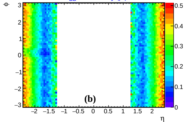
Trigger Efficiency ( \mu^- )
