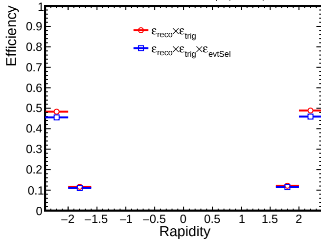
Coherent J/\psi (0n0n)
