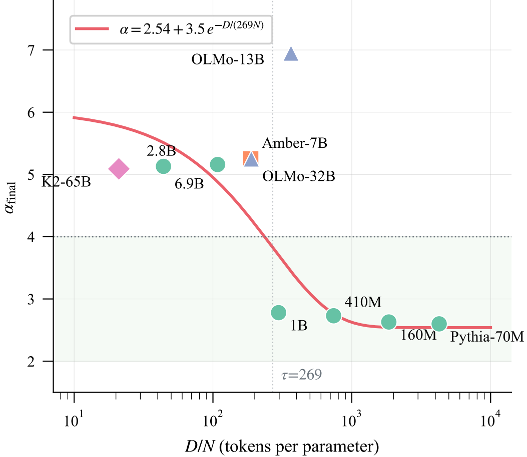
Figure 6: Structural Chinchilla: \alpha_{\text{final}} vs. D/N . The original exponential formula (red curve) fits small models ( \leq 7\text{B} ) but fails for larger models. OLMo-2-13B is a strong outlier ( \alpha = 6.95 at D/N = 365 ), revealing that model size N enters as an independent variable.
