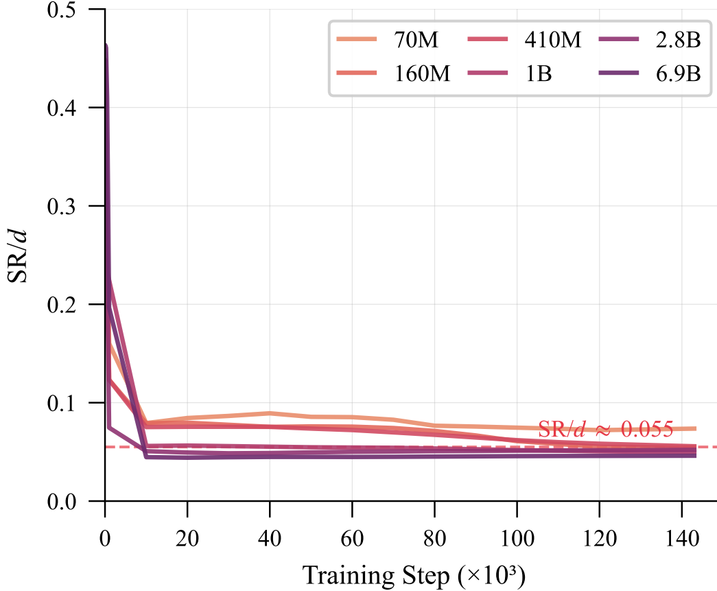
Figure 1: SR/d convergence during training across 6 Pythia scales. Despite 100\times variation in model size, all trajectories converge to the universal band SR/d \approx 0.05\text{--}0.07 .
