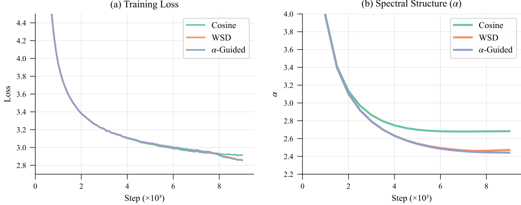
Figure 3: Three-way schedule comparison (mean of 2 seeds). (a) Training loss: WSD and \alpha -Guided converge to lower loss than cosine. (b) Spectral structure: cosine’s \alpha plateaus after step 5K due to premature LR decay, while WSD and \alpha -Guided continue structural improvement.
