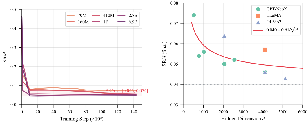
(a) \text{SR}/d convergence during training across 6 Pythia scales. All trajectories converge to the universal band \text{SR}/d \approx 0.05\text{--}0.07 .
