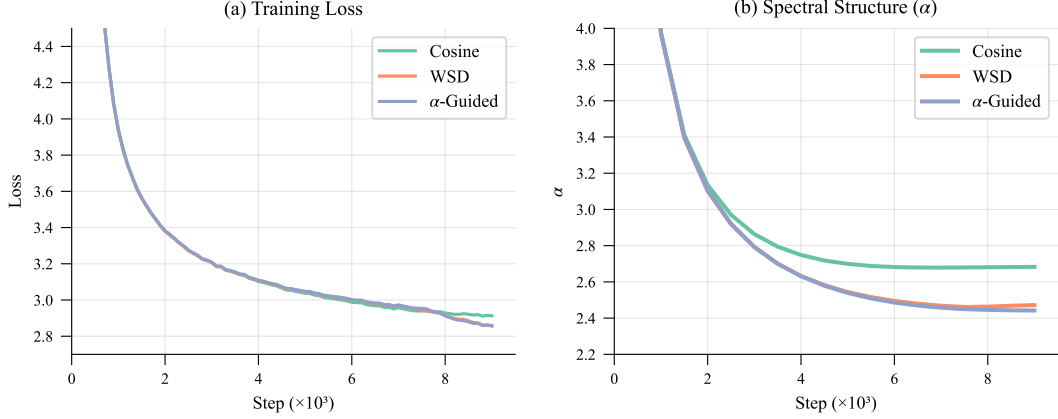
Figure 6: Three-way schedule comparison (mean of 2 seeds). (a) Training loss: WSD and \alpha -Guided converge to lower loss than cosine. (b) Spectral structure: cosine’s \alpha plateaus after step 5K due to premature LR decay, while WSD and \alpha -Guided continue structural improvement.
