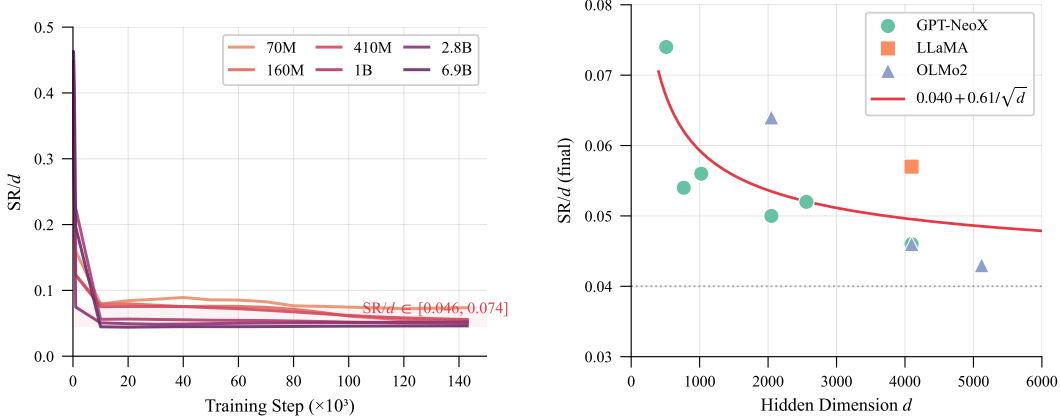
(a) SR/d convergence during training across 6 Pythia scales. All trajectories converge to the universal band SR/d \approx 0.05\text{--}0.07 .
