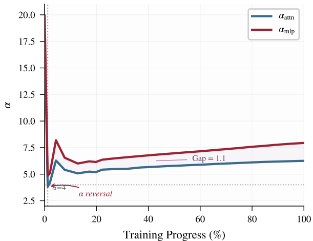
(b) OLMo-2-13B: MLP vs Attention
