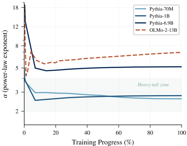
(a) Overall \alpha trajectories
