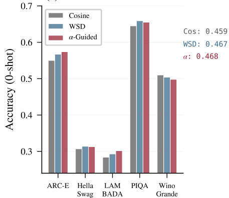
(c) Downstream Benchmarks
