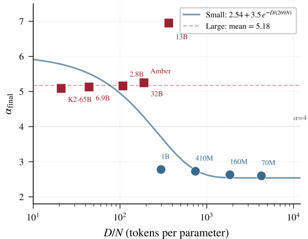
(a) \alpha vs Data Ratio D/N
