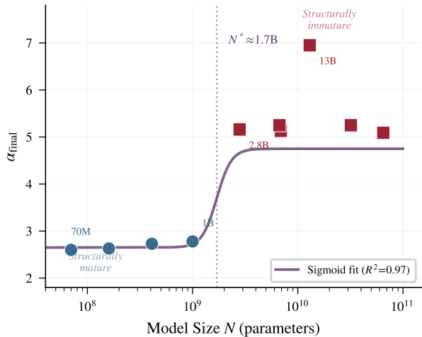
(b) Phase Transition at N^* \approx 1.7\text{B}
