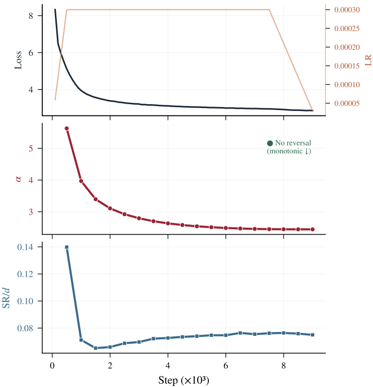
\alpha -Guided Training Monitor (Pythia-410M)
