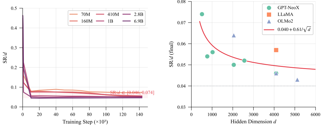
(a) \text{SR}/d convergence during training across 6 Pythia scales. All trajectories converge to the universal band \text{SR}/d \approx 0.05\text{--}0.07 .
