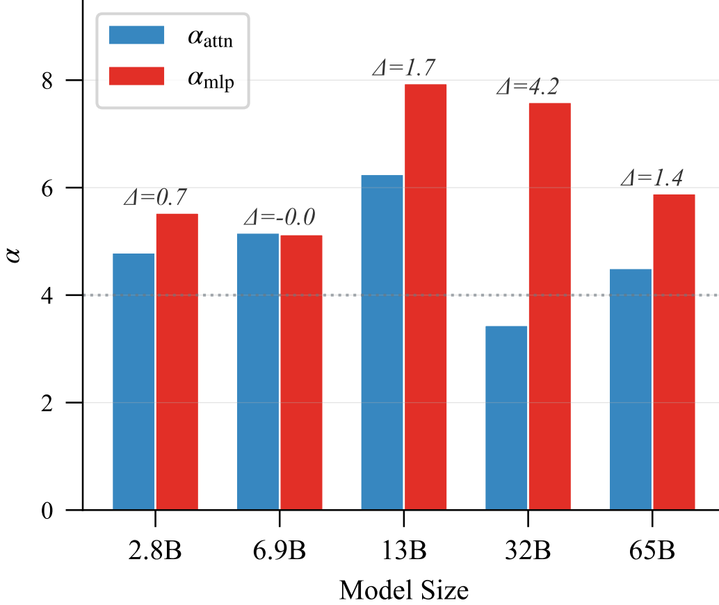
Figure 4: MLP vs. Attention \alpha decomposition for models exhibiting reversal. The gap \Delta = \alpha_{\text{mlp}} - \alpha_{\text{attn}} amplifies at scale, reaching 4.2 at 32B. At 32B, attention layers achieve heavy-tail structure ( \alpha_{\text{attn}} = 3.4 < 4 ) while MLP layers remain structurally immature ( \alpha_{\text{mlp}} = 7.6 ).
