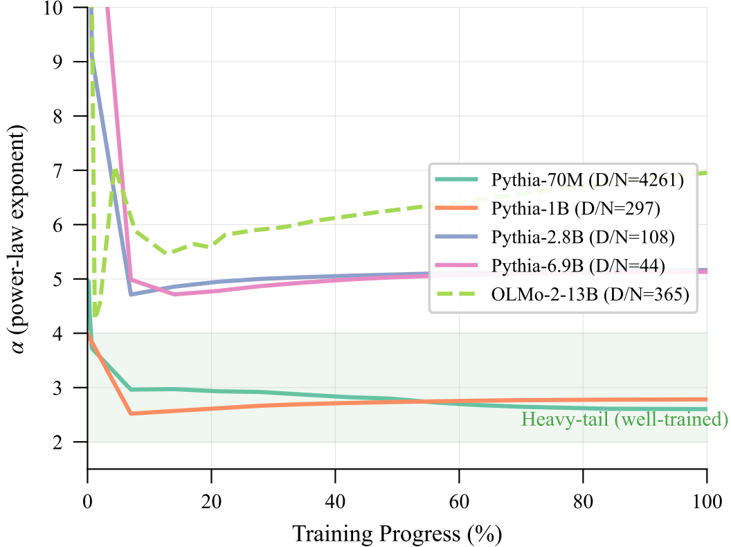
Figure 3: \alpha dynamics during training. Well-trained models (70M, 1B) converge into the heavy-tail regime ( \alpha < 4 ). Under-trained models (2.8B, 6.9B, 13B) exhibit \alpha reversal: initial structure formation followed by degradation. OLMo-2-13B shows the strongest reversal ( \Delta\alpha = +2.71 ) despite having D/N = 365 .
