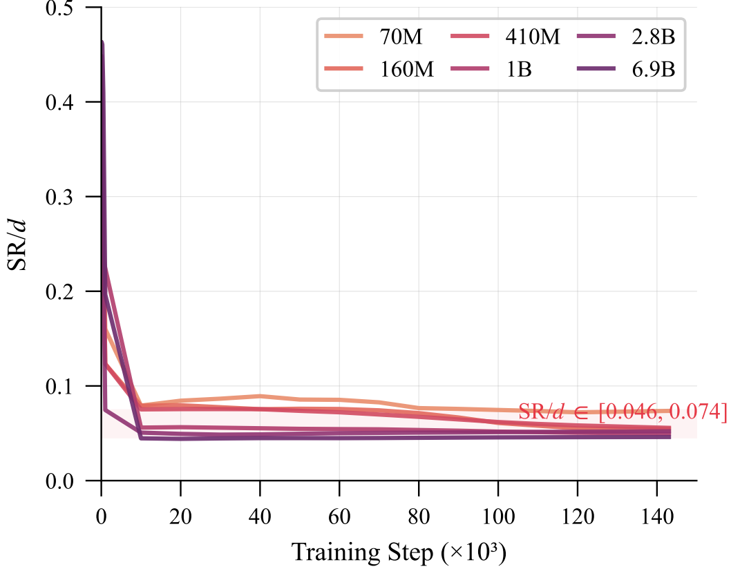
Figure 1: SR/d convergence during training across 6 Pythia scales. Despite 100\times variation in model size, all trajectories converge to the universal band SR/d \approx 0.05\text{--}0.07 .
