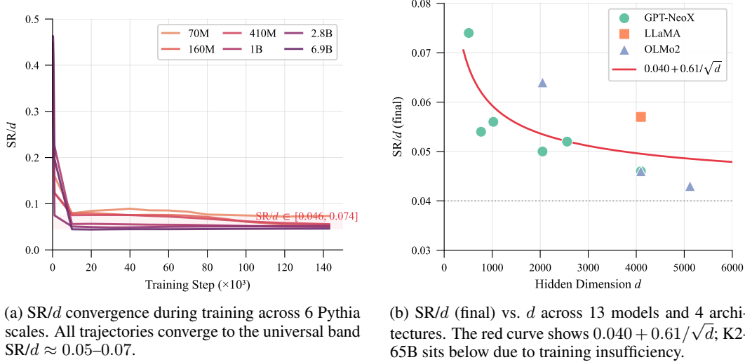
Figure 2: Universal compression law. (a) Despite 100\times variation in model size, SR/d converges to a narrow band determined by hidden dimension d . (b) The asymptotic model SR/d \approx 0.040 + 0.61/\sqrt{d} fits all 13 models across 4 architecture families; deviations reflect training insufficiency, not architectural differences.
