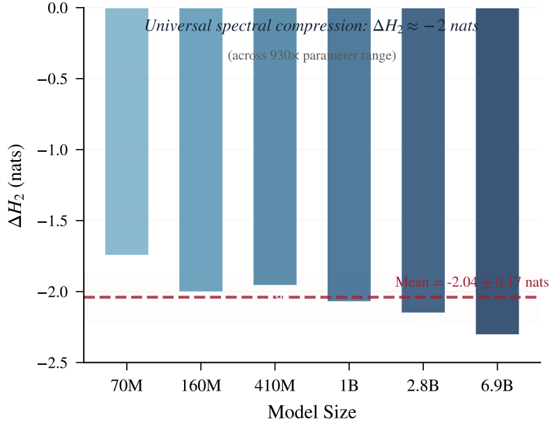
Figure 11: Universal spectral compression: every sufficiently-trained model removes \Delta H_2 \approx -2 nats of Rényi-2 entropy per layer, regardless of scale (70M–6.9B). The dashed line shows the mean ( -2.04 \pm 0.17 nats).
