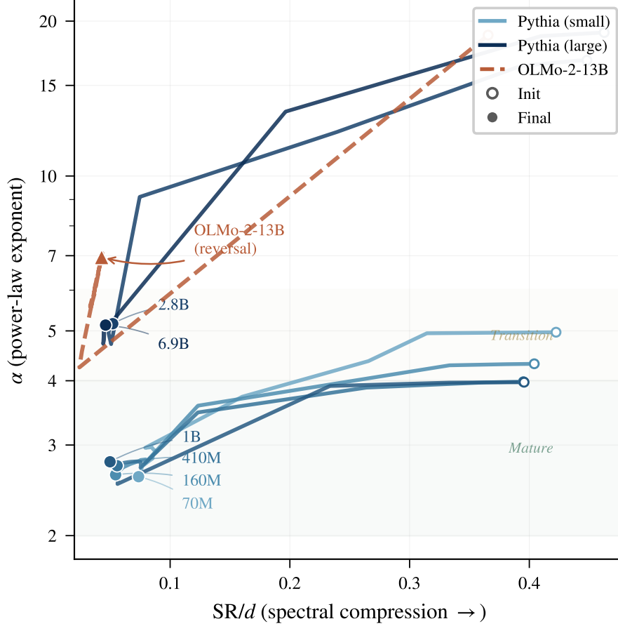
Figure 1: Spectral phase portrait. Each model traces a trajectory through (\text{SR}/d, \alpha) space during training (right=init, left=final). Well-trained small models (70M–1B) converge to the lower-left “mature” region ( \alpha < 4 , \text{SR}/d < 0.08 ). Under-trained large models (2.8B, 6.9B) stall in the “transition” zone. OLMo-2-13B reverses direction after reaching its \alpha minimum, moving away from maturity. All models share the same compression axis ( \text{SR}/d converges universally) but diverge on the structural quality axis ( \alpha ).
