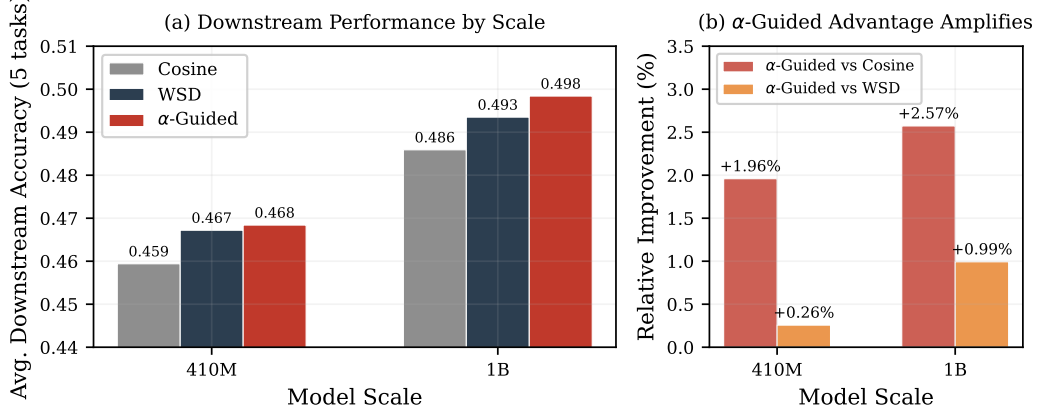
Figure 7: α-guided advantage amplifies with scale. (a) Downstream accuracy (5 benchmarks) for three schedules at 410M and 1B. (b) Relative improvement of α-guided: the gap vs. cosine grows from +1.96% to +2.57%, and vs. WSD from +0.26% to +0.99%. Larger models benefit more from adaptive decay timing.
