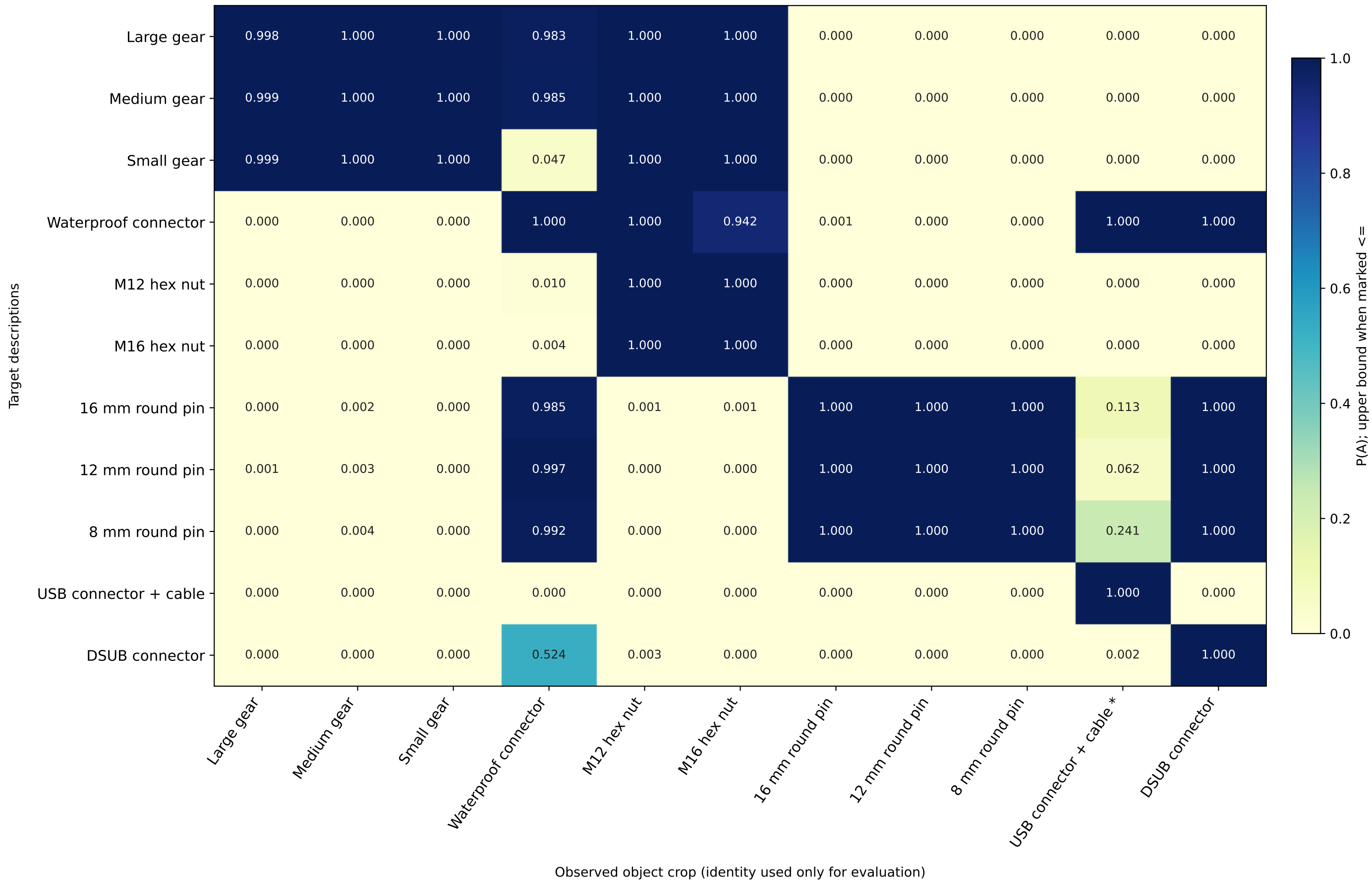
Scene 303: gemma4:12b P(A)
