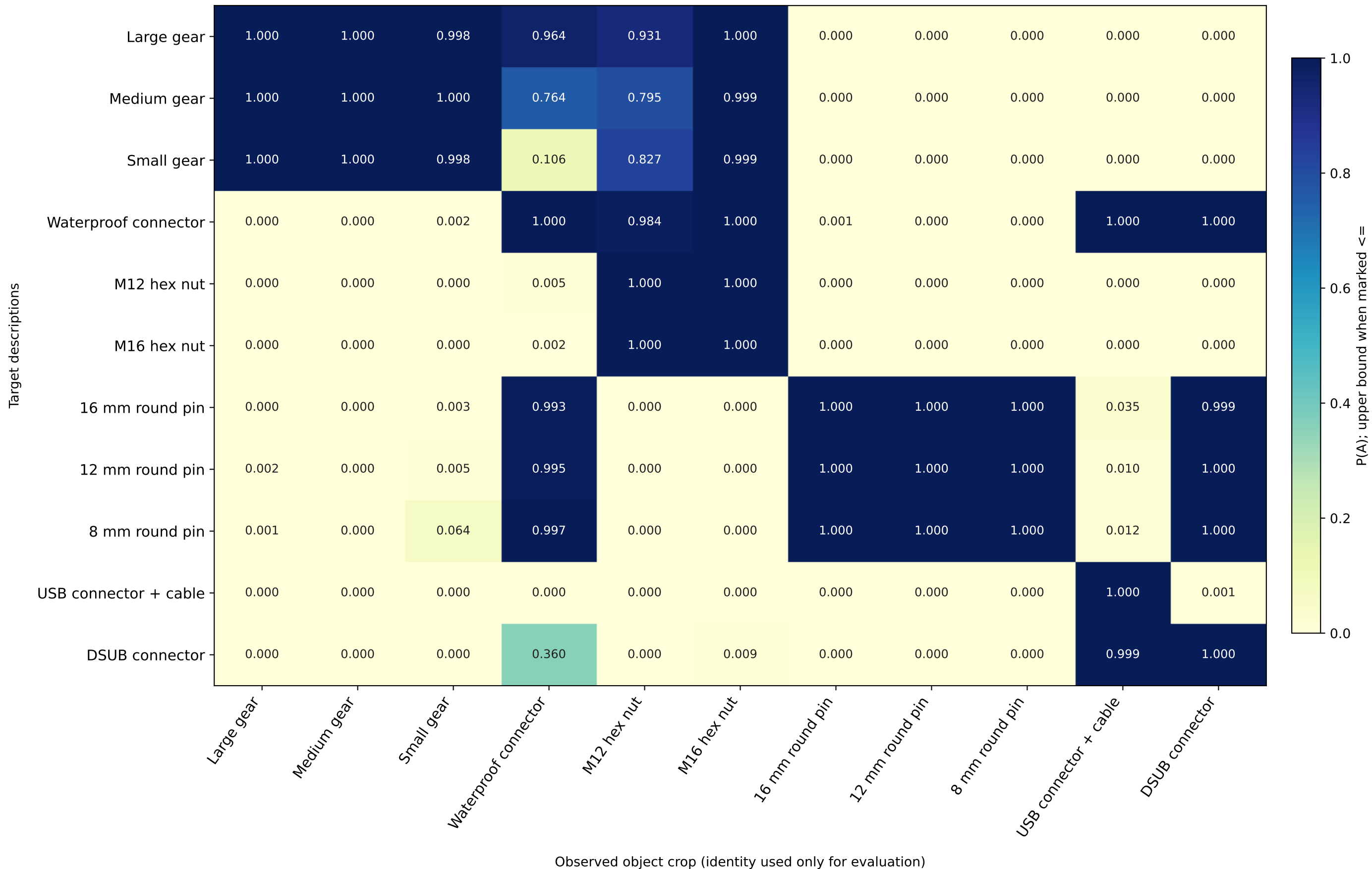
Scene 202: gemma4:12b P(A)
